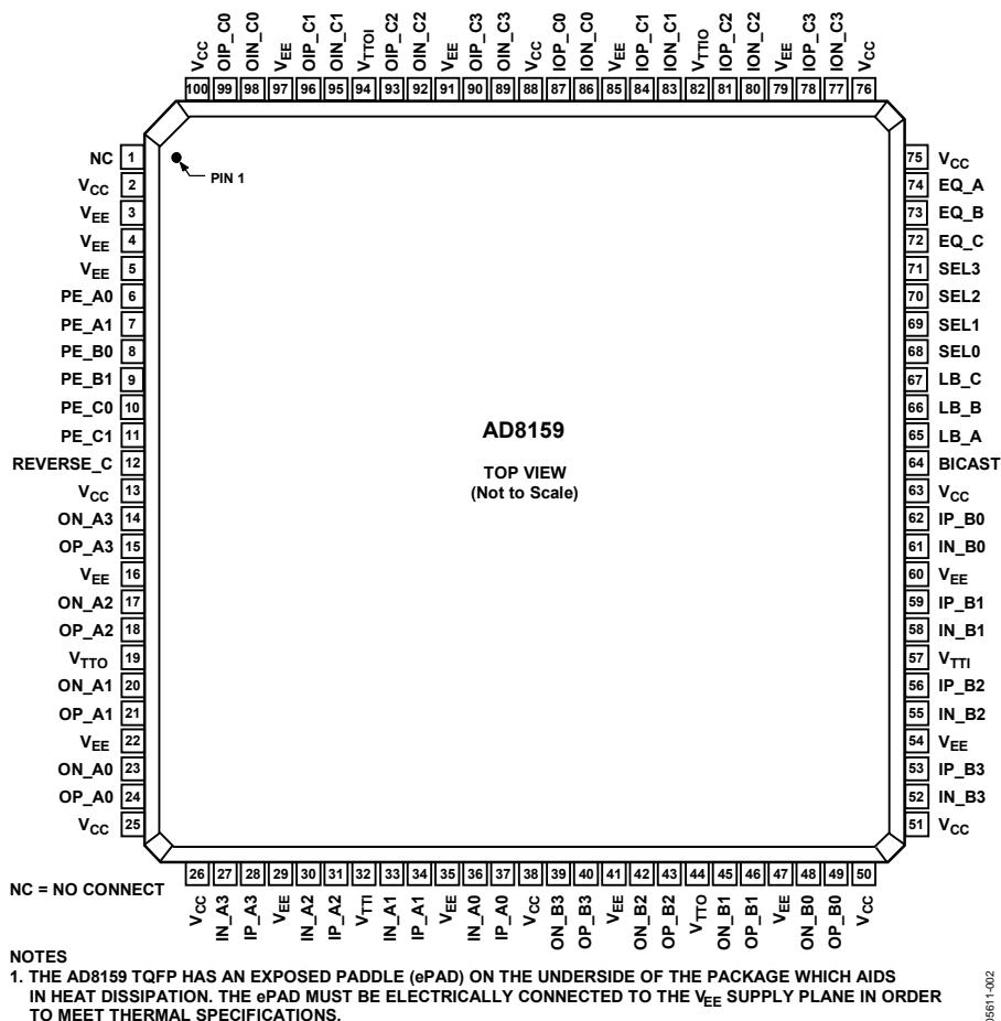
Figure 2. Pin Configuration
