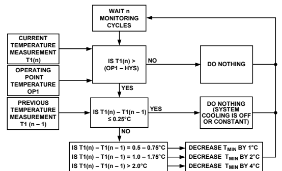
Figure 67. Short Cycle Steps
