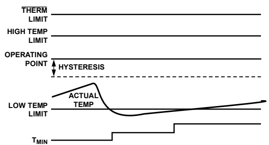
Figure 71. Increasing T MIN for Quieter Operation
