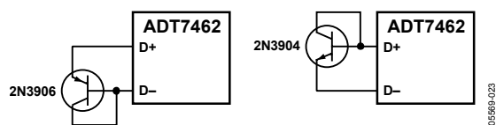
Figure 33. How to Measure Temperature Using Discrete Transistors
