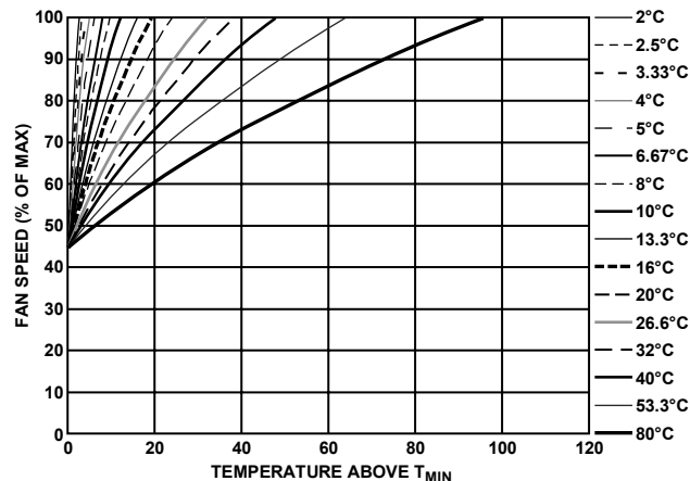
Figure 60. T_{RANGE} and % Fan Speed Slopes with PWM_{MIN} = 20\%
