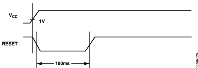
Figure 84. Operation of \overline{\text{RESET}} Output on Power-Up
