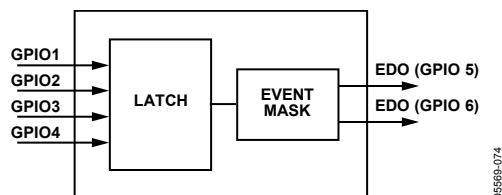
Figure 83. EDO Circuit
