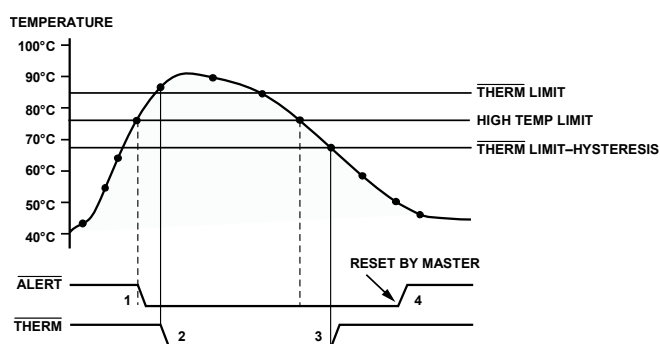
Figure 82. \overline{\text{THERM}} Behavior
