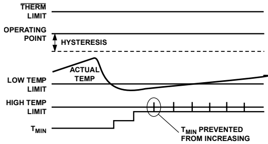
Figure 72. T_{MIN} Adjustments Limited by High Temperature Limit
