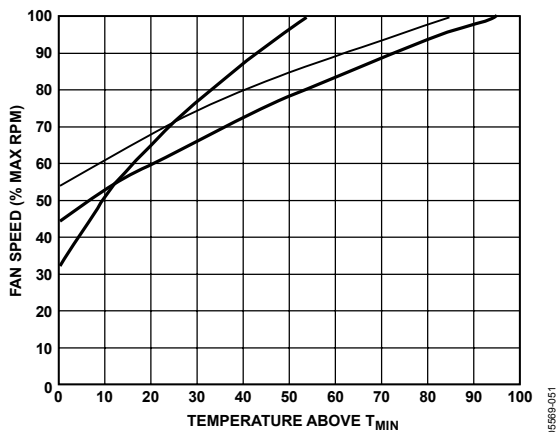
Figure 61. T_{\text{RANGE}} and % Fan Speed Slopes for VRM, Ambient, and CPU Temperature Channels
