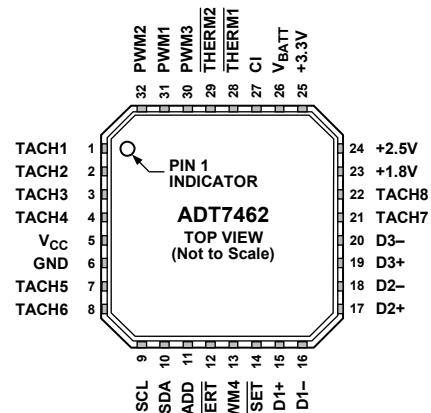
Figure 4. Configuration Option 1
