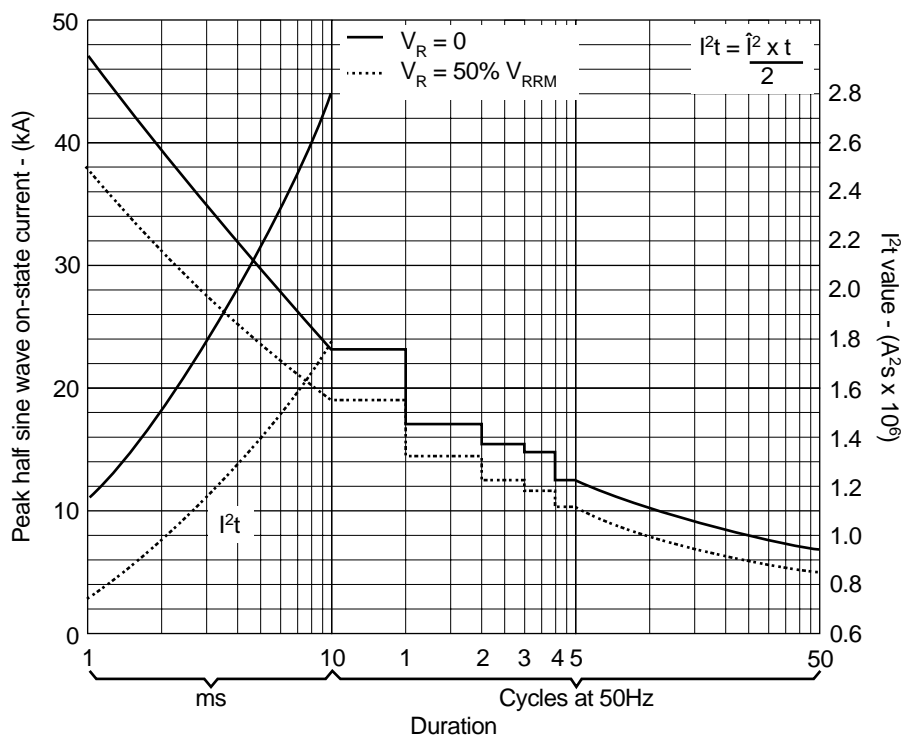
Fig.6 Surge (non-repetitive) on-state current vs time at T_{case} 125^{\circ}C
