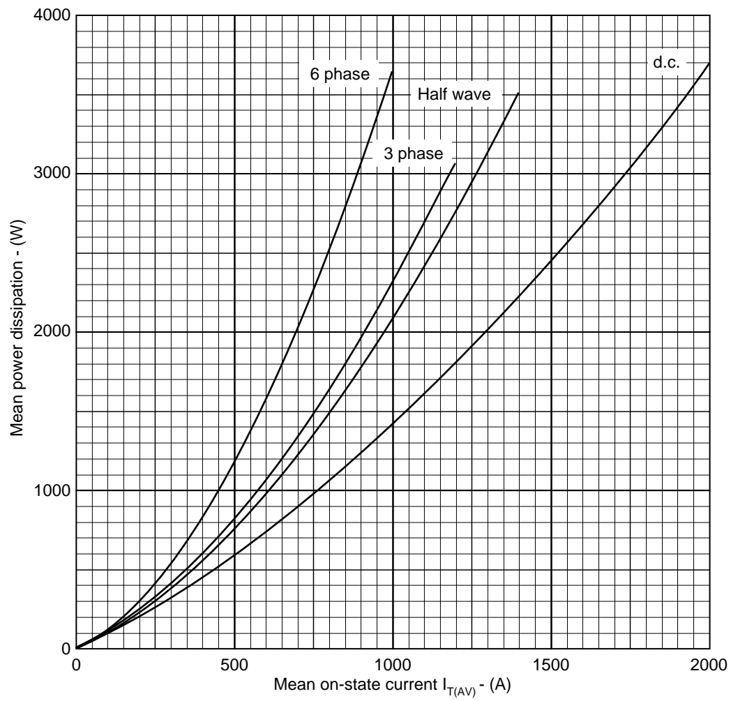
Fig.2 Dissipation curves
