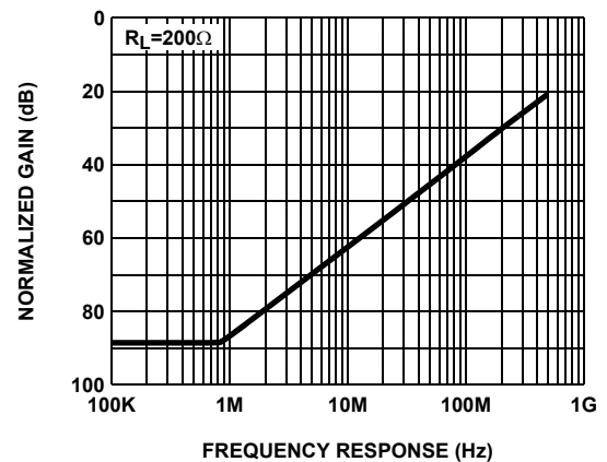
FIGURE 6. CMRR
