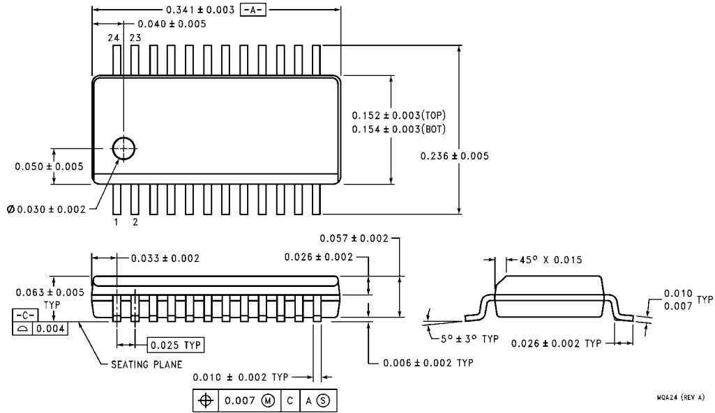
24-Lead Quarter Size Outline Package (QSOP), JEDEC MO-137, 0.150\"/>
