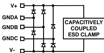
CIRCUIT 4
