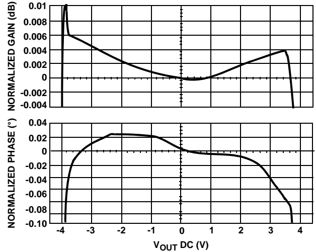
FIGURE 14. DIFFERENTIAL GAIN AND PHASE; V_{OUT} = 0.2V_{P-P} , F_O = 3.58MHz , R_L = 150\Omega
