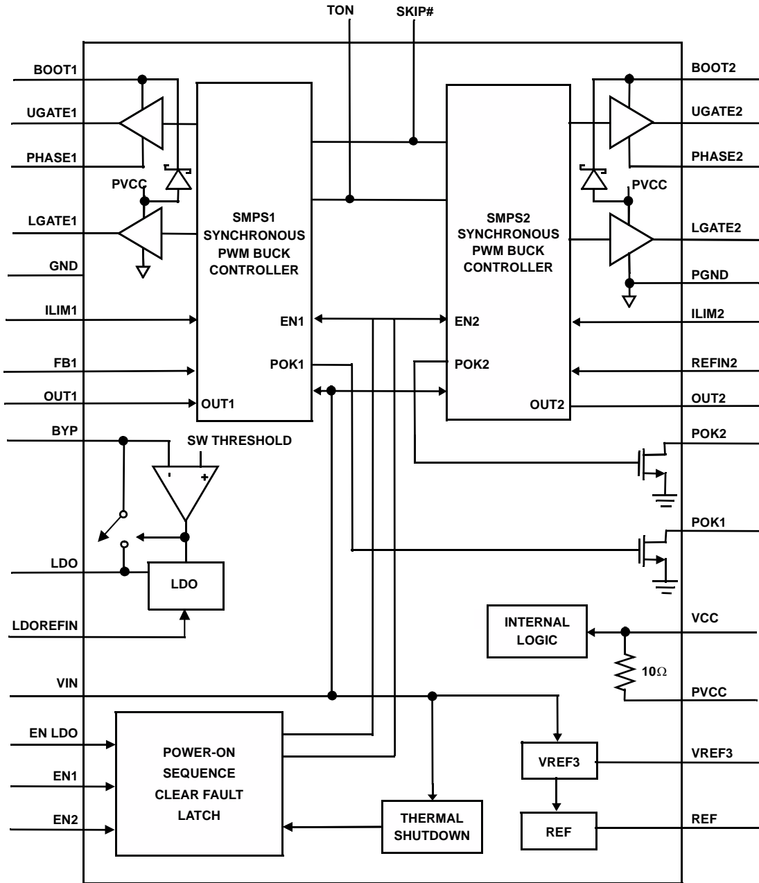
FIGURE 70. DETAIL FUNCTIONAL DIAGRAM ISL6236A
