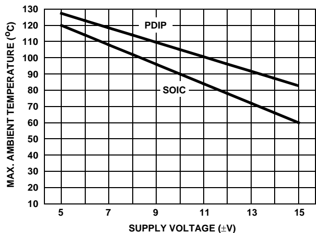
FIGURE 7. MAXIMUM OPERATING AMBIENT TEMPERATURE vs SUPPLY VOLTAGE
