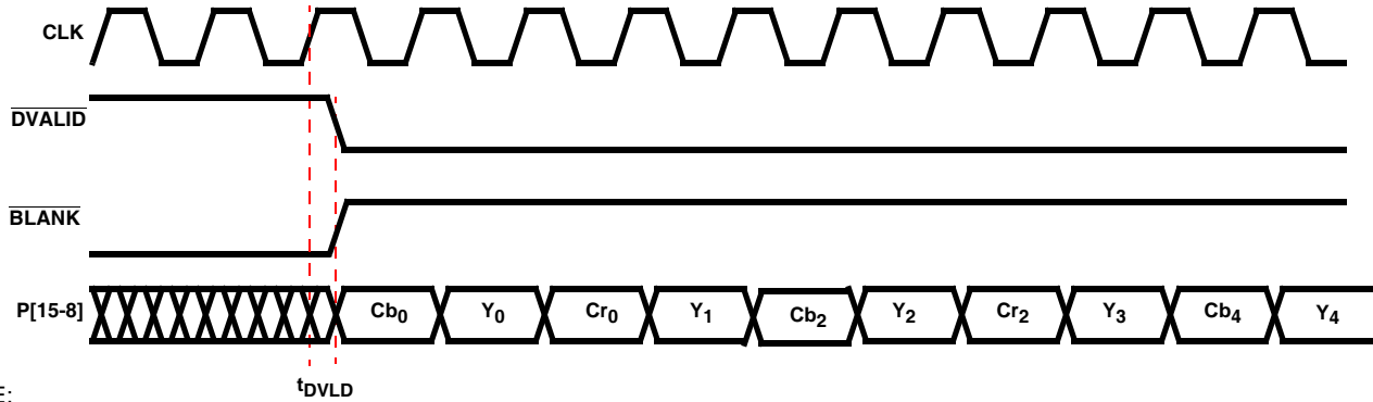
FIGURE 8. OUTPUT TIMING FOR 8-BIT YCbCr MODE (DVLDT_LTC = 0)
