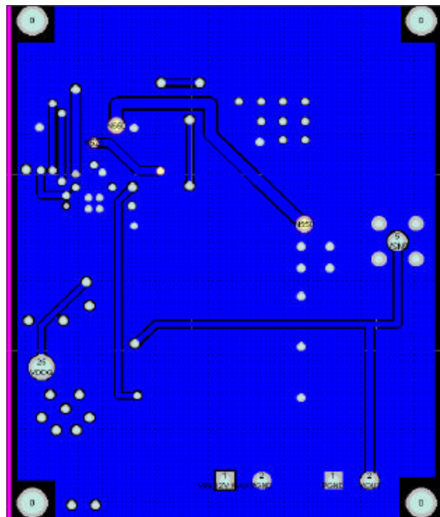
Figure 2.4 - Bottom layer.
