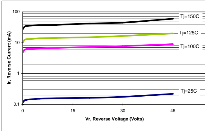
Figure 1: Typical Reverse Current (per leg)
