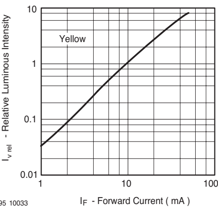
Figure 17. Relative Luminous Intensity vs. Forward Current
