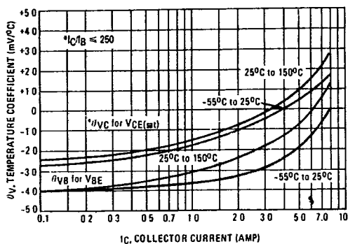
FIGURE 12 - TEMPERATURE COEFFICIENTS
