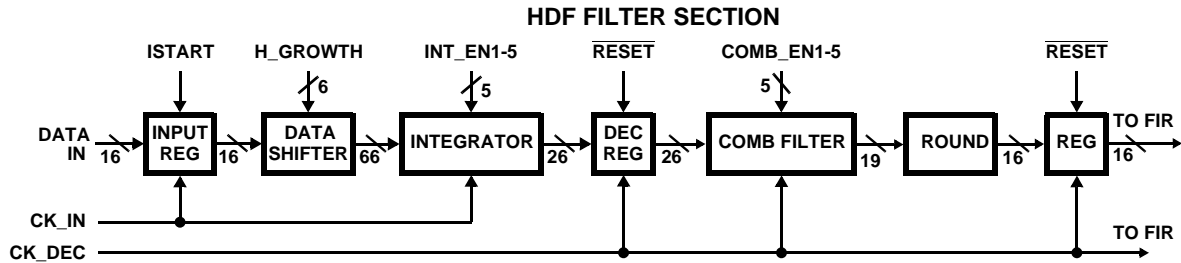
FIGURE 1. HIGH ORDER DECIMATION FILTER FIGURE
