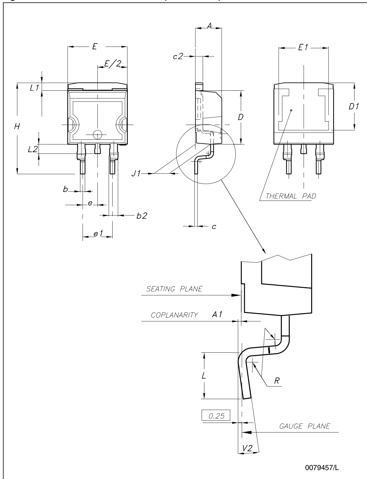
Figure 7. DRAWING DIMENSION D 2 PAK (TYPE STD-ST)
