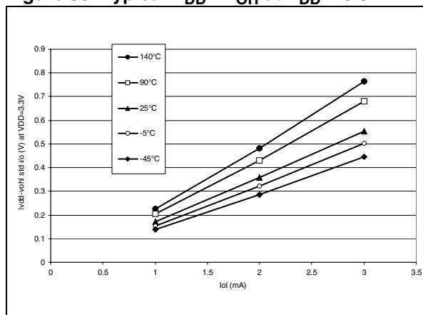
Figure 86. Typical V_{DD} - V_{OH} at V_{DD} = 5V
