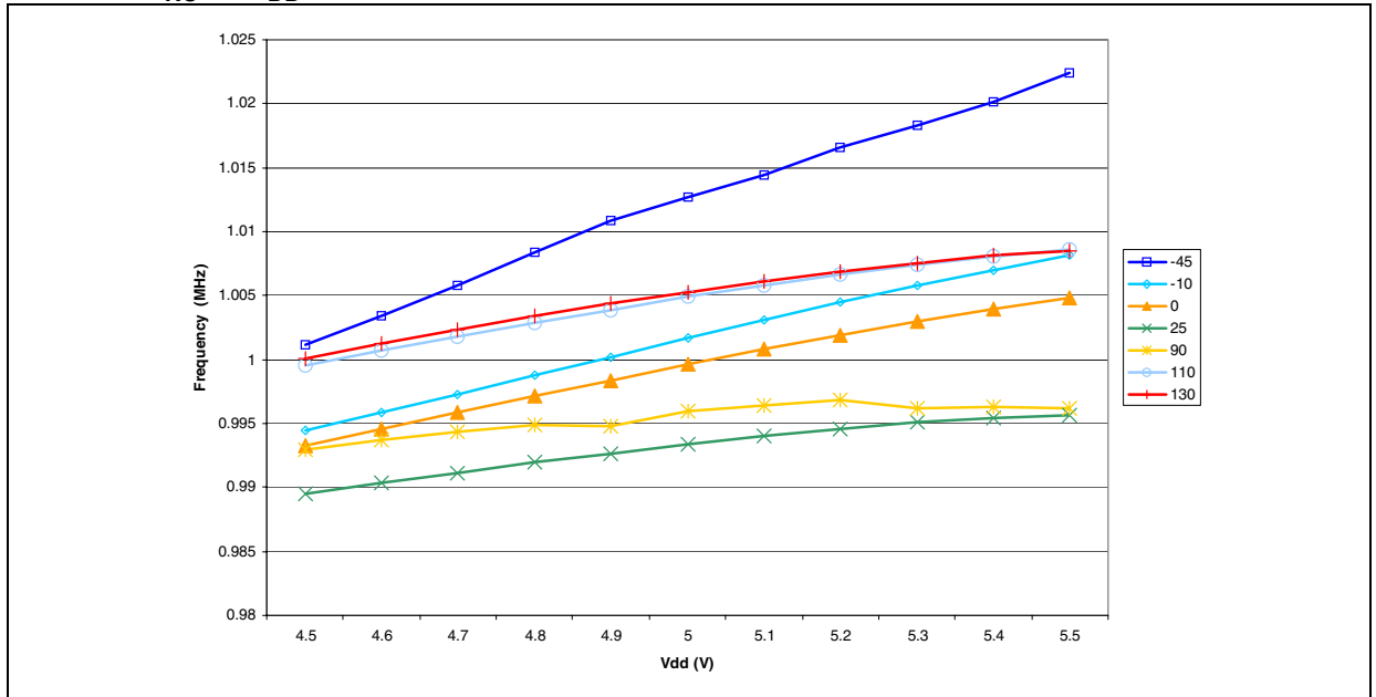
Figure 62. f_{RC} vs V_{DD} and Temperature for Calibrated RCCR0
