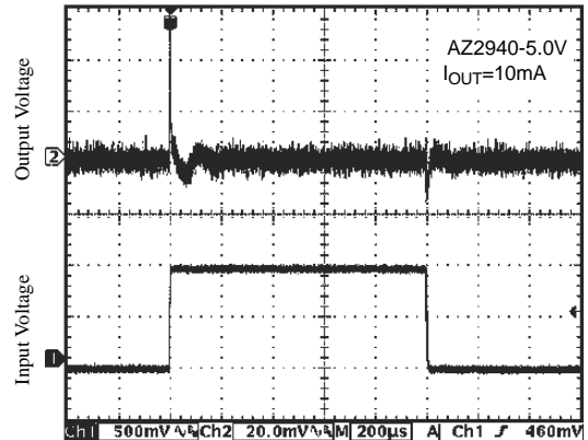
Figure 19. Line Transient
