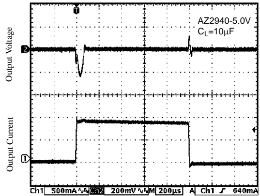
Figure 17. Load Transient
