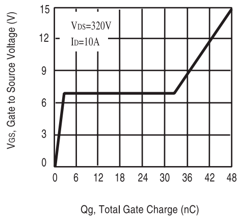
Figure 9. Gate Charge
