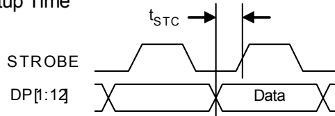
Setup Time
