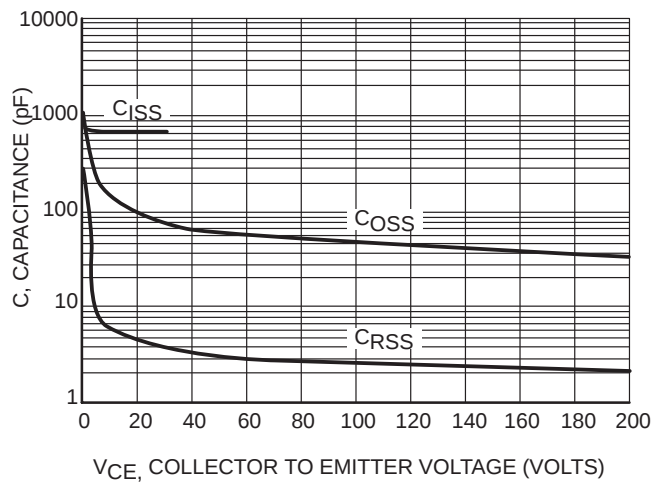
Figure 5. Capacitance Variation
