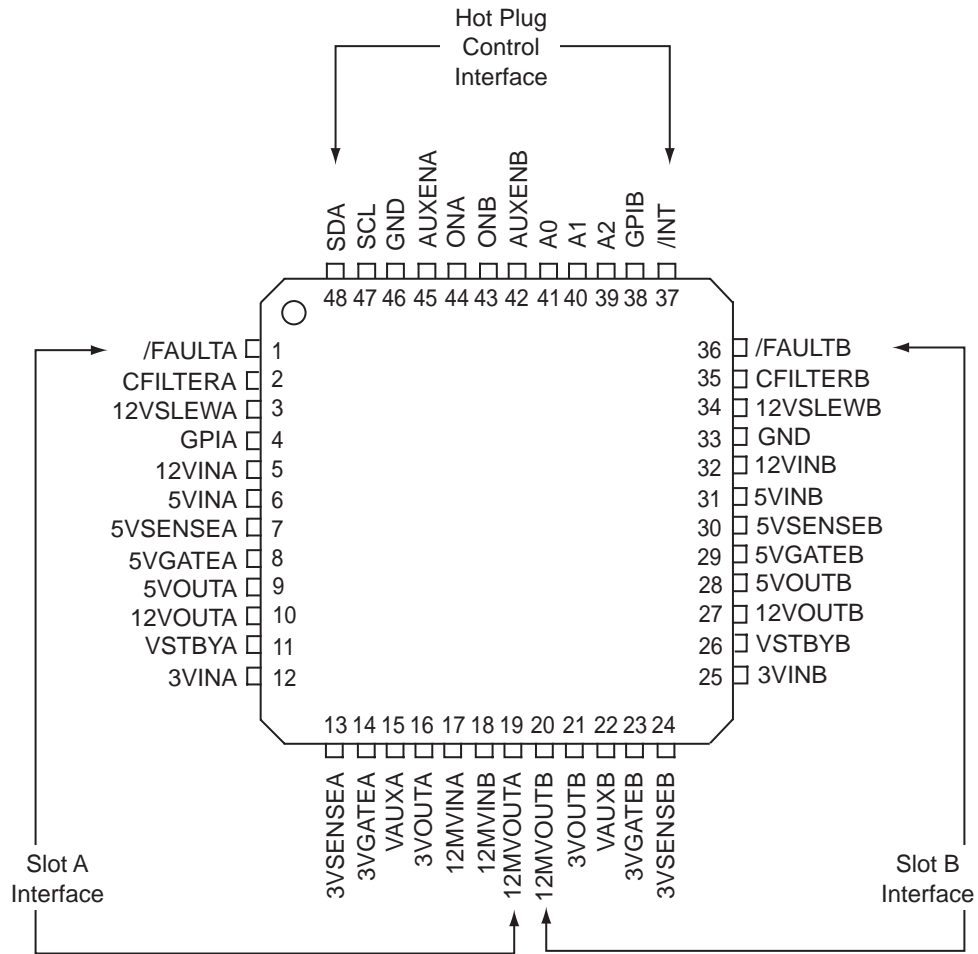
48-Pin TQFP
