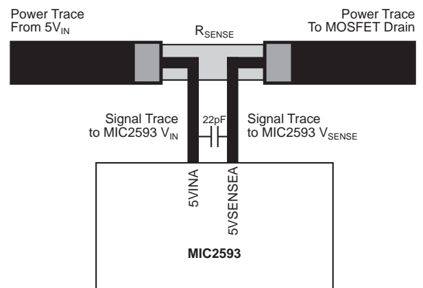
Figure 12. Kelvin Sense Connections for R_{SENSE} (Applicable to 5V[A/B] and 3V[A/B])
