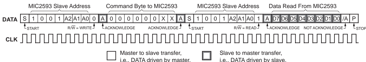
Figure 10. READ_BYTE Protocol
