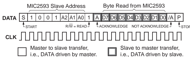
Figure 11. RECEIVE_BYTE Protocol
