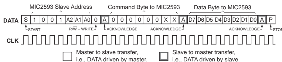
Figure 9. WRITE_BYTE Protocol
