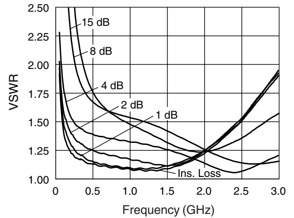
VSWR vs. Frequency (-40°C)
