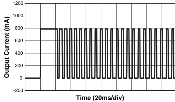
Over-Current Protection
