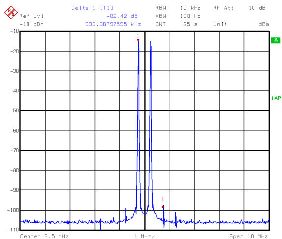
FIGURE 11. TWO TONES (CkxF=6) AT 8.5MHz, 50MSPS CLOCK, 500kHz SPACING (82dBc - 10MHz WINDOW, 6dB PAD)
