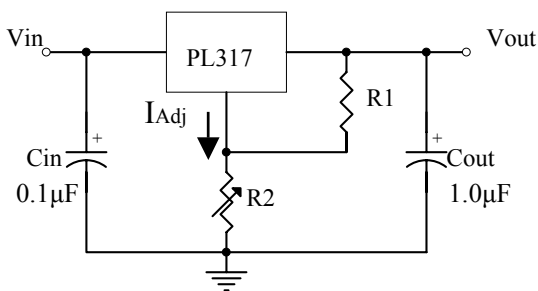
Standard Application
