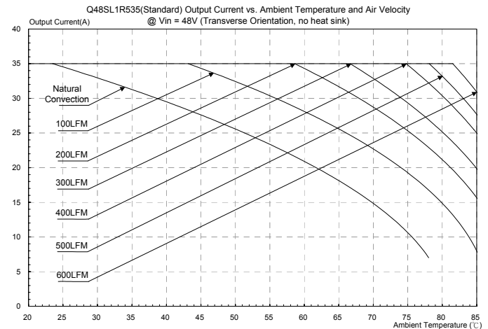
Figure 22: Q48SL1R535NR (Standard) Output current vs. ambient temperature and air velocity@Vin=48V (Transverse orientation, no heat sink).
