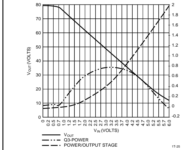
FIGURE 2. CVA1556N DC CHARACTERISTICS
