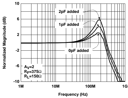
Frequency Response for Various C_{IN}
