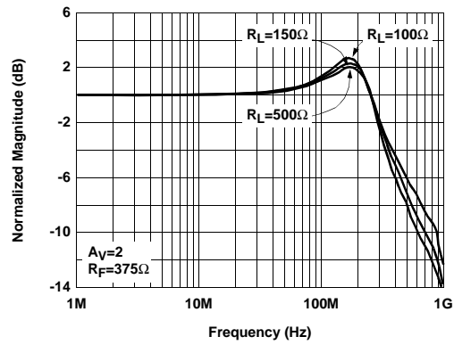
Frequency Response for Various R_L
