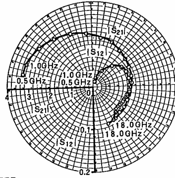
S_{12}, S_{21} vs. f
