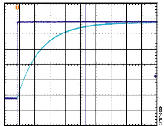
Figure 20. Turn-On Time – C_X, C_Y = 0.1 \mu F , Time Scale = 2 ns/div
