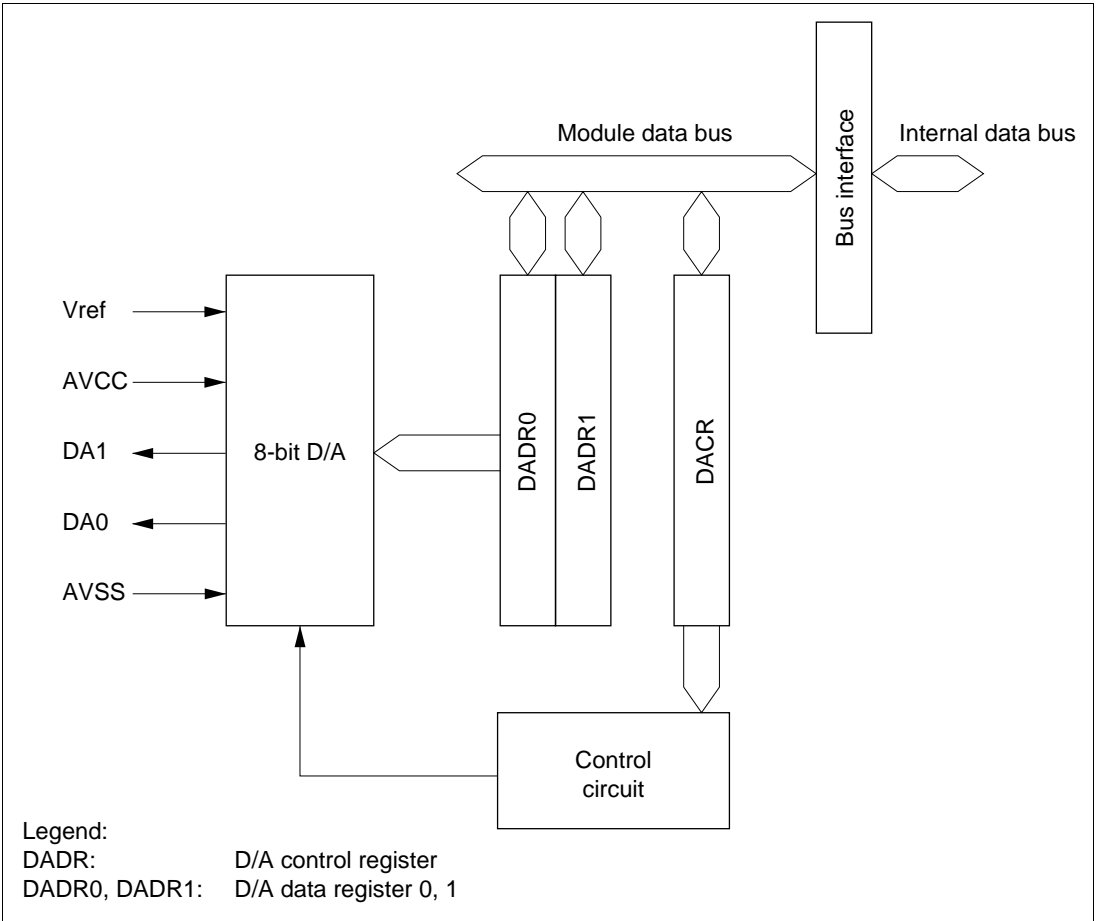
Figure 18-1 Block Diagram of D/A Converter
