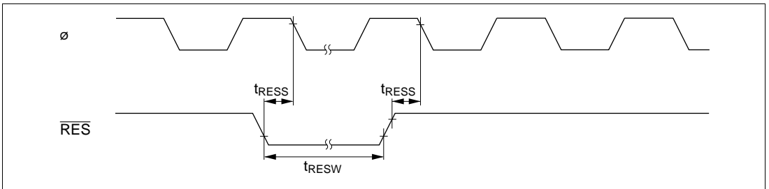
Figure 24-9 Reset Input Timing
