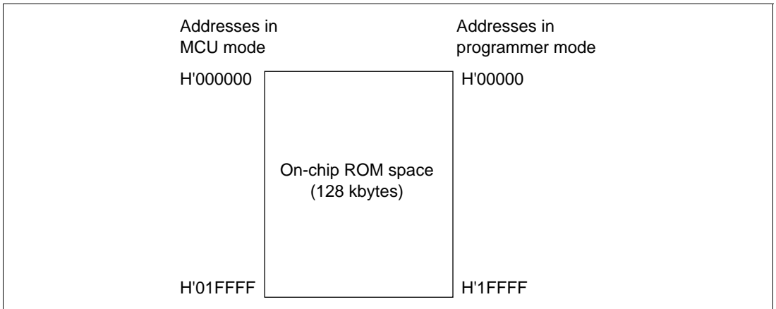
Figure 21A-17 On-Chip ROM Memory Map
