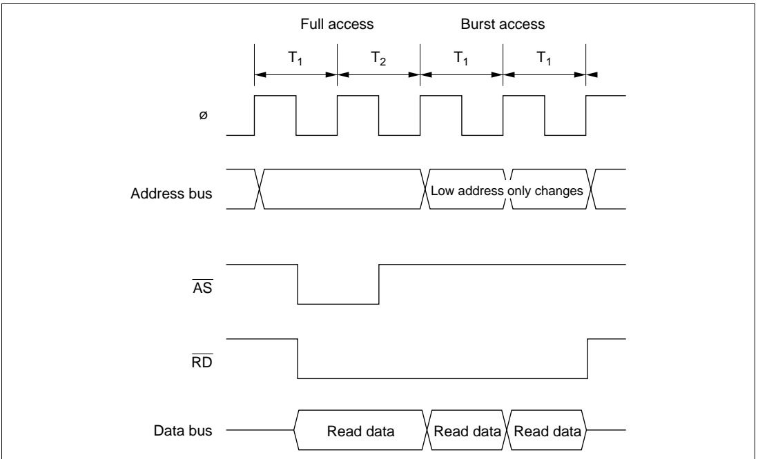
Figure 7-14 (b) Example Burst ROM Access Timing ( AST0=BRSTS1=0 )
