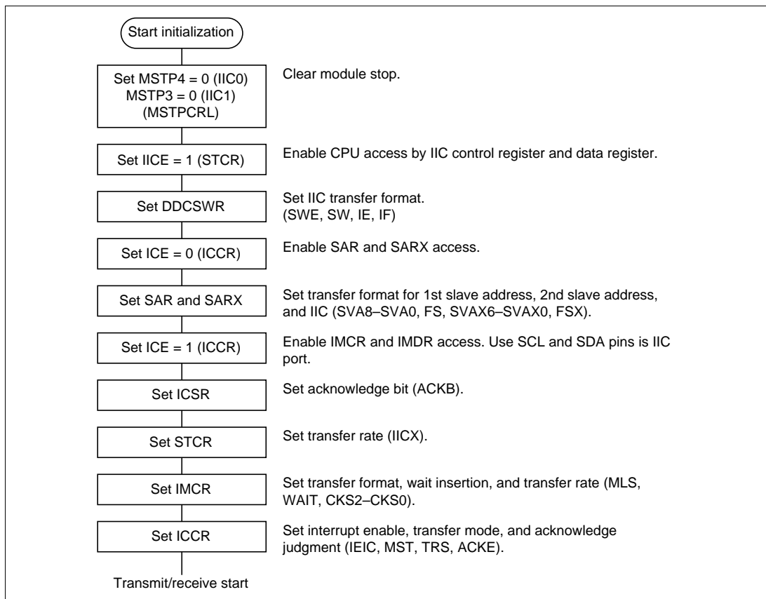
Figure 15-6 Flowchart for IIC Initialization (Example)
