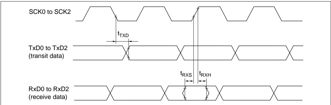
Figure 24-23 SCI Input/Output Timing (Clock Synchronous Mode)
