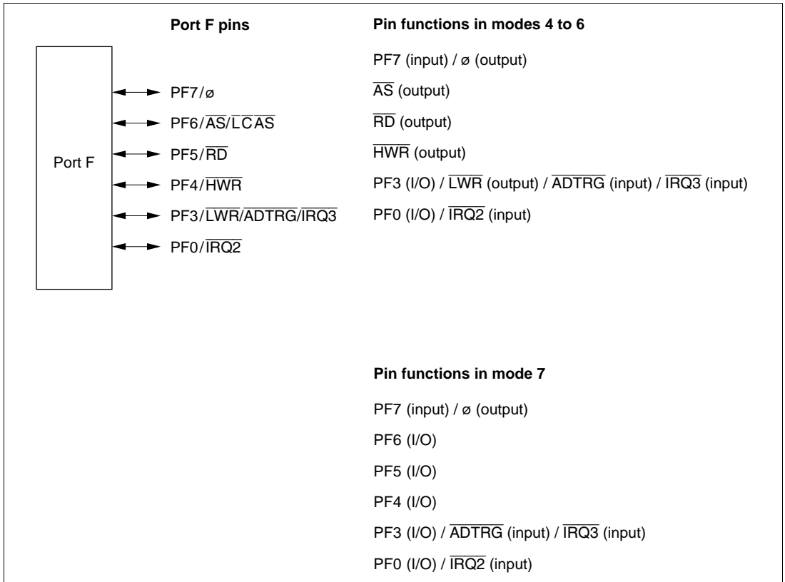
Figure 9-21 Port F Pin Functions
