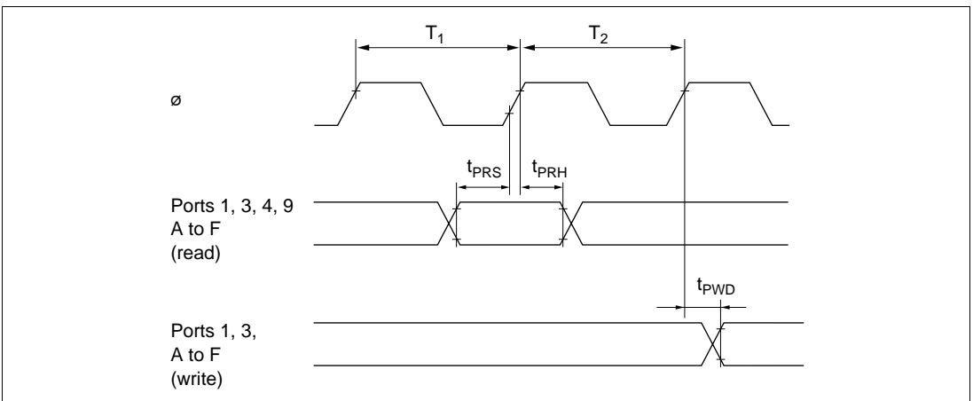
Figure 24-16 I/O Port Input/Output Timing (Ports 1, 3, 4, 9, A to F)
