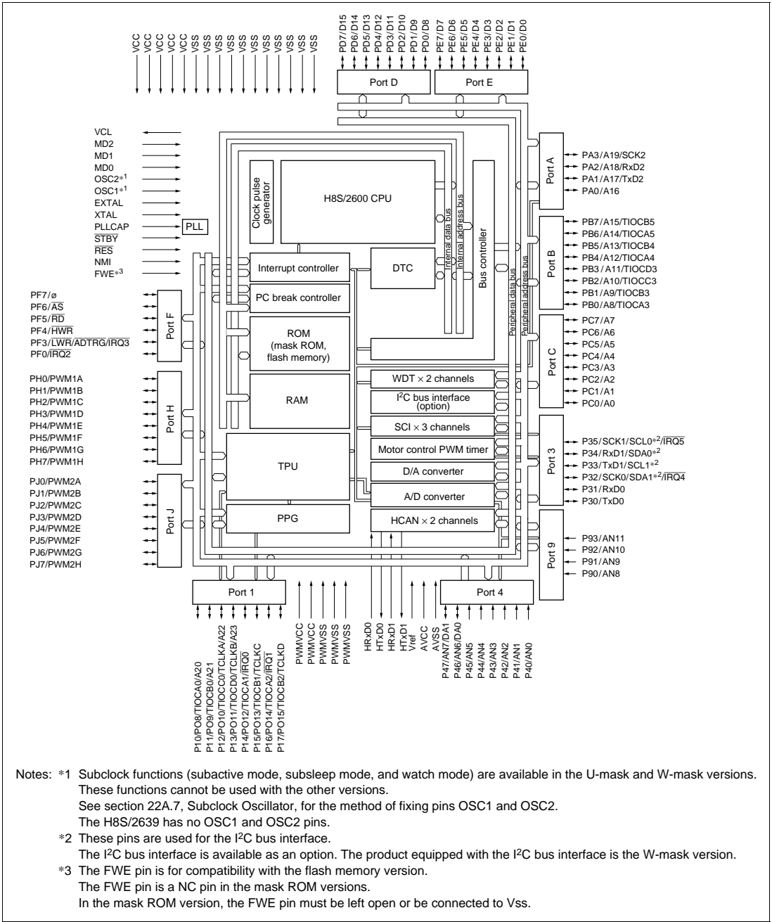
Figure 1-1 (b) Internal Block Diagram of H8S/2638 and H8S/2639
