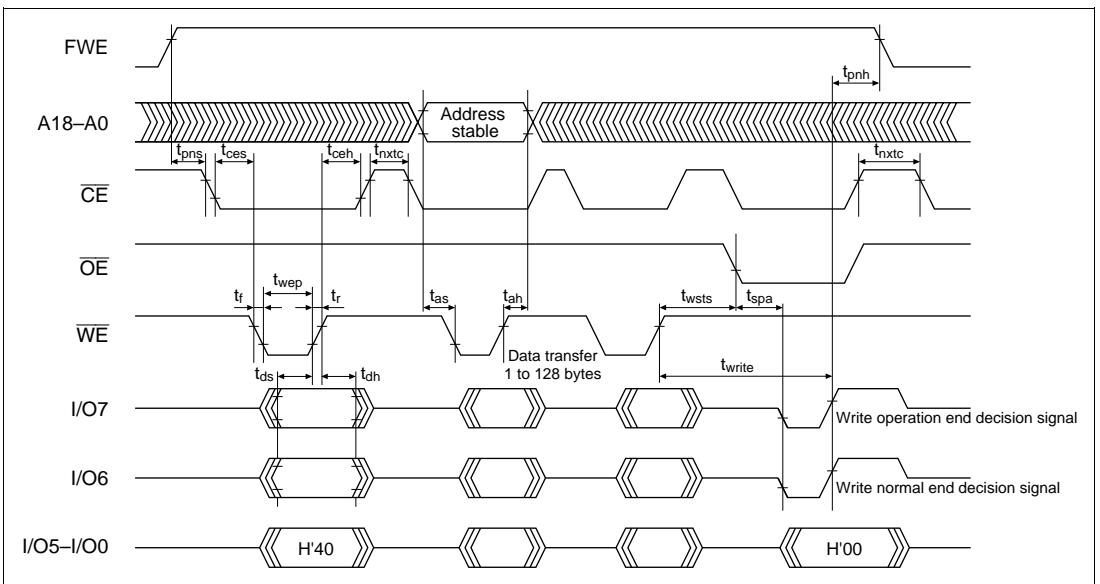
Figure 21B-22 Auto-Program Mode Timing Waveforms
