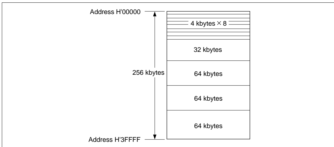
Figure 21B-6 Flash Memory Block Configuration
