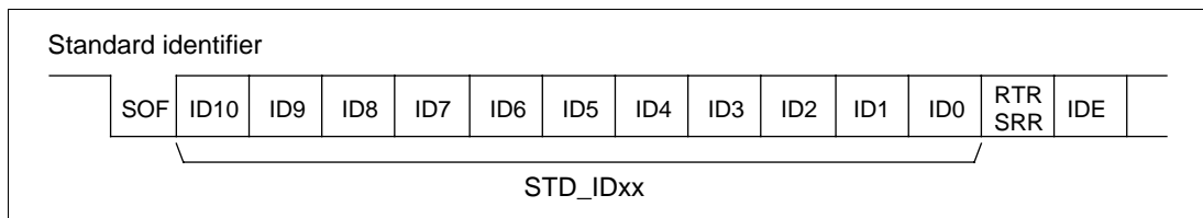
Figure 16-2 Standard identifier
