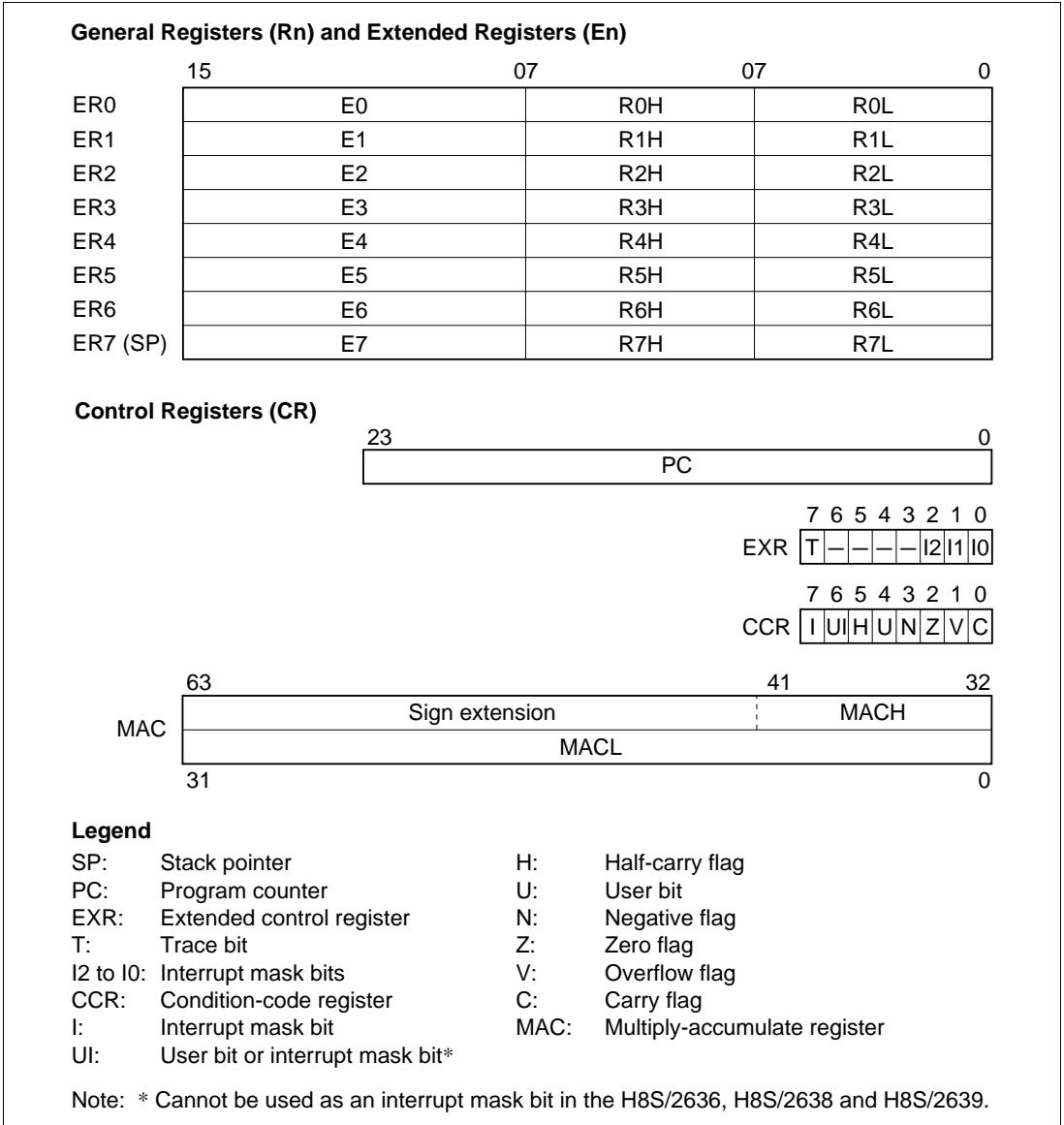
Figure 2-7 CPU Registers
