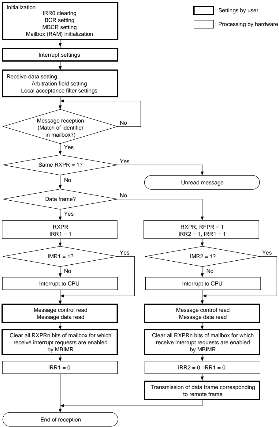
Figure 16-9 Reception Flowchart
