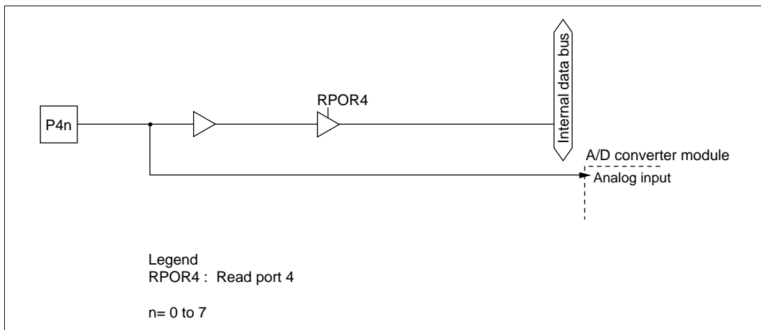
Figure C-3 Port 4 Block Diagram (Pins P40 to P47)
