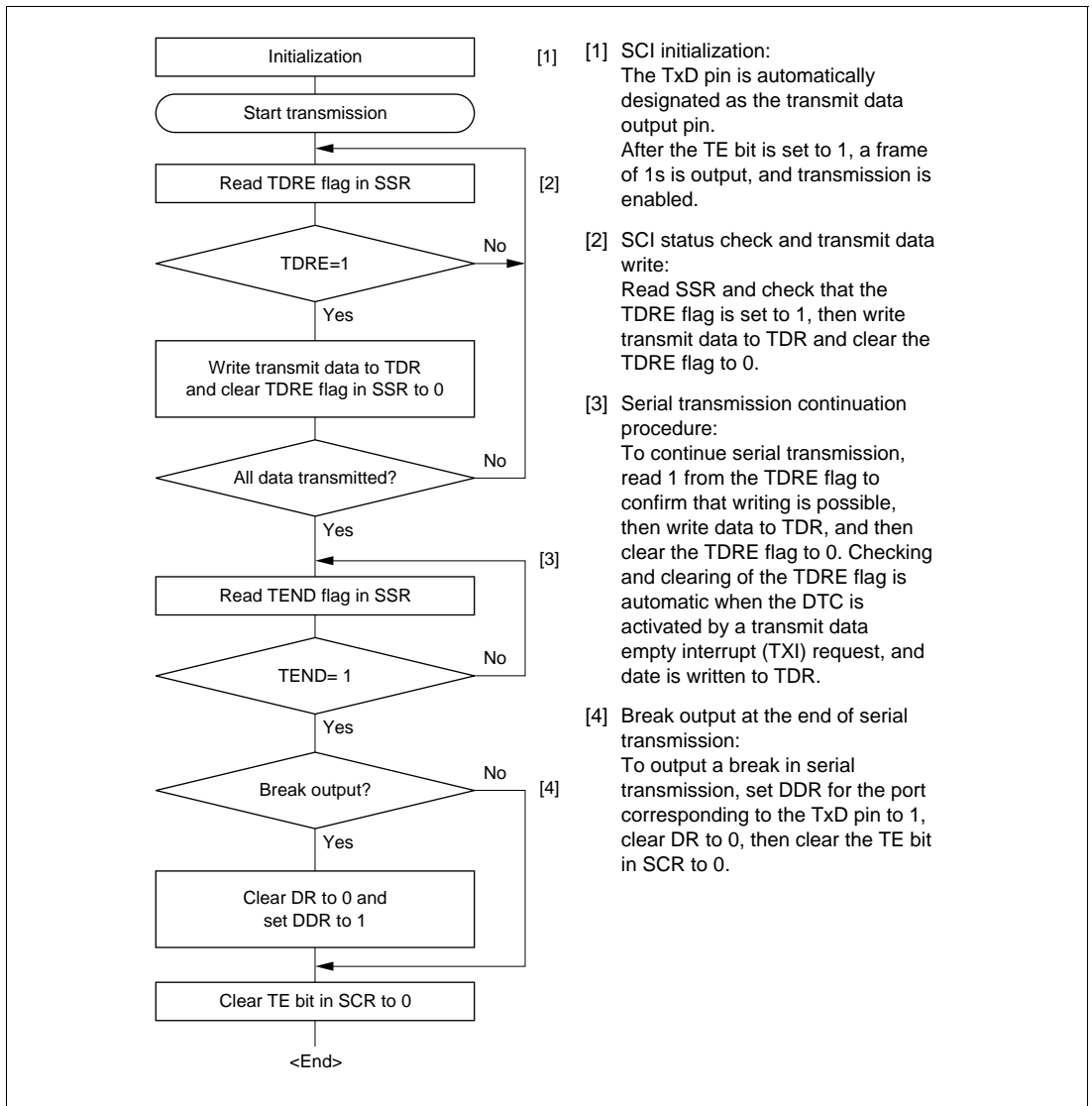
Figure 13-5 Sample Serial Transmission Flowchart
