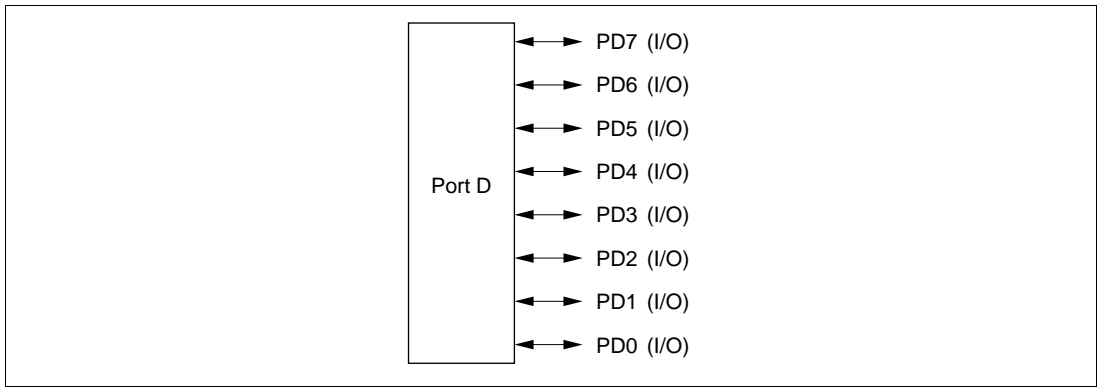
Figure 9-17 Port D Pin Functions (Mode 7)
