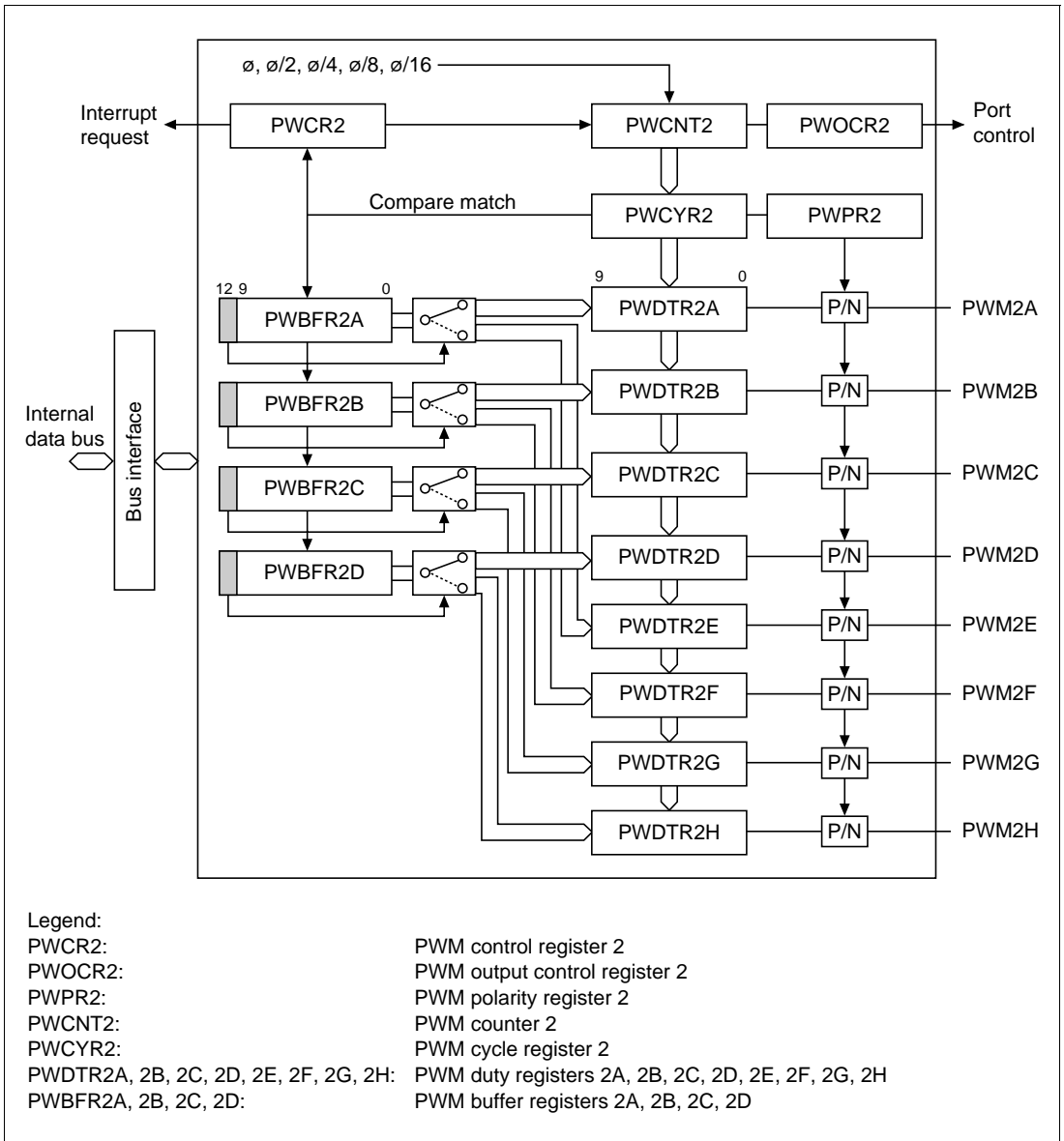
Figure 19-2 Block Diagram of PWM Channel 2
