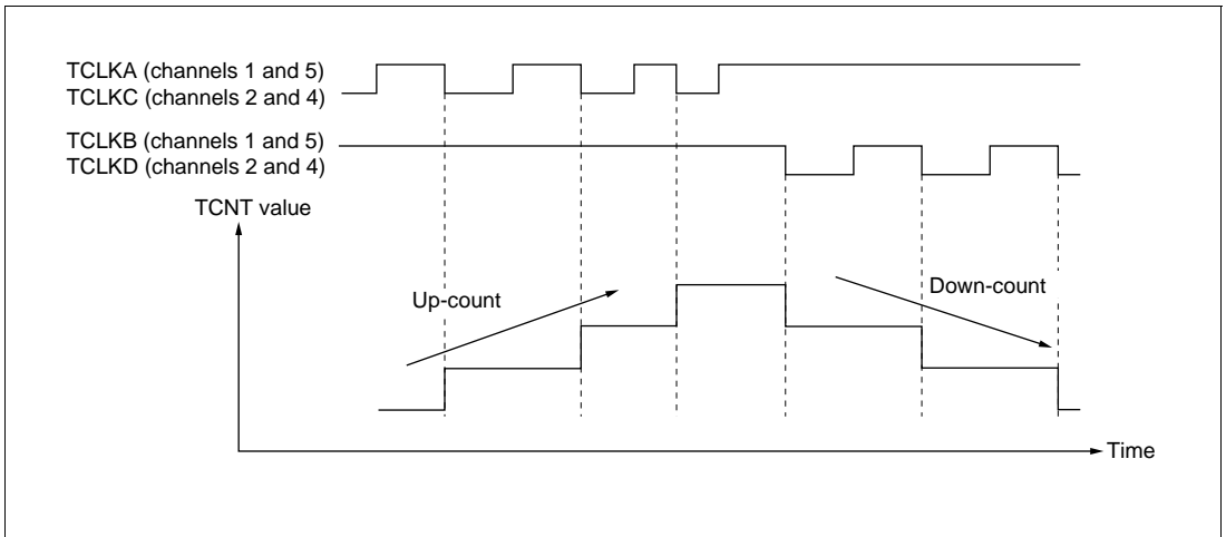
Figure 10-31 Example of Phase Counting Mode 3 Operation
