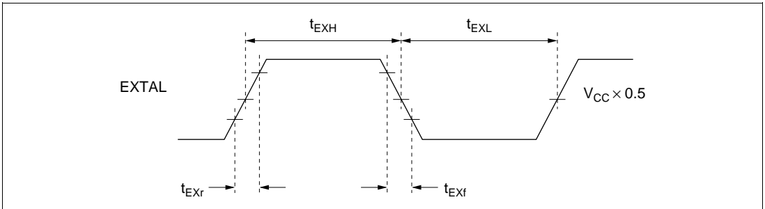
Figure 22B-7 External Clock Input Timing
