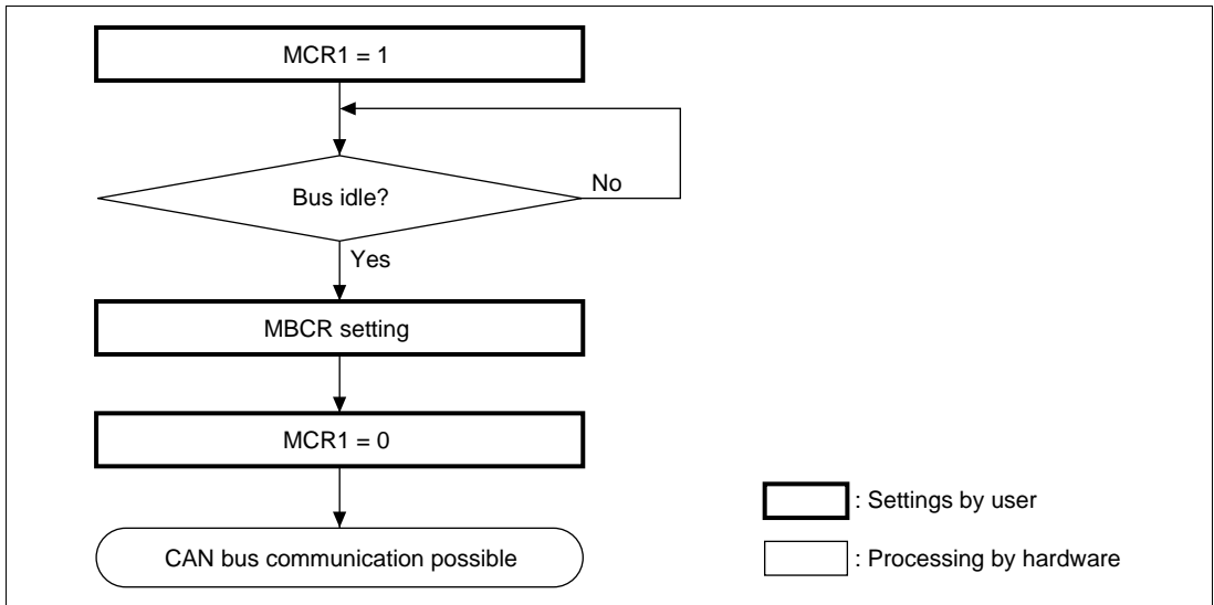
Figure 16-12 HCAN Halt Mode Flowchart
