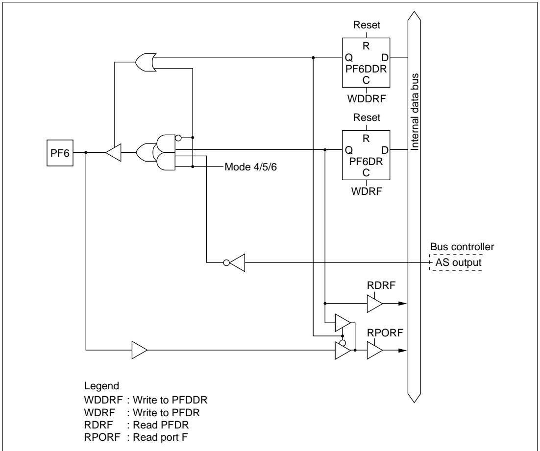
Figure C-10 (e) Port F Block Diagram (Pin PF6)
