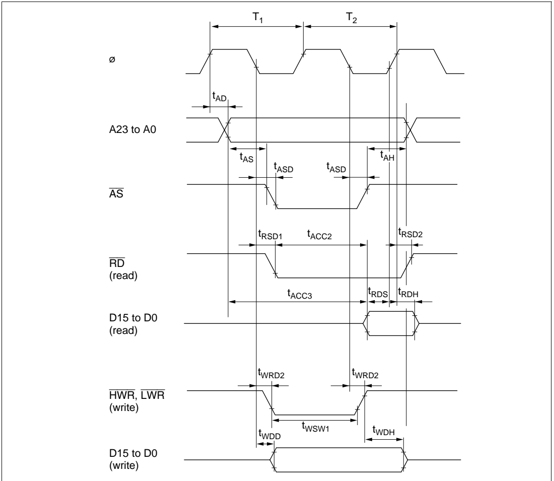
Figure 24-11 Basic Bus Timing (Two-State Access)
