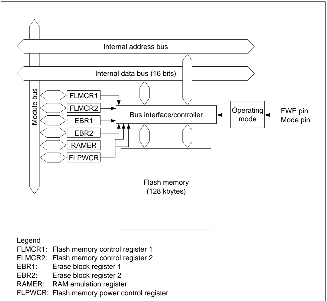
Figure 21A-2 Block Diagram of Flash Memory
