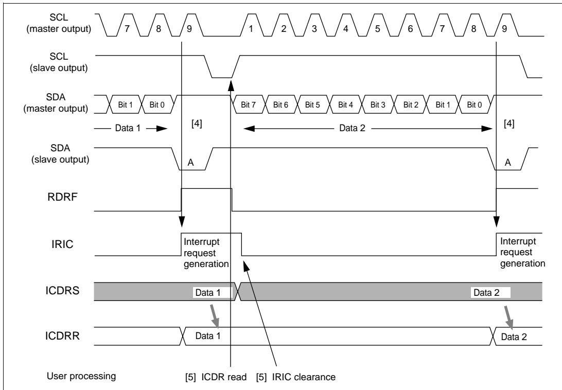
Figure 15-15 Example of Slave Receive Mode Operation Timing (2) (MLS = ACKB = 0)
