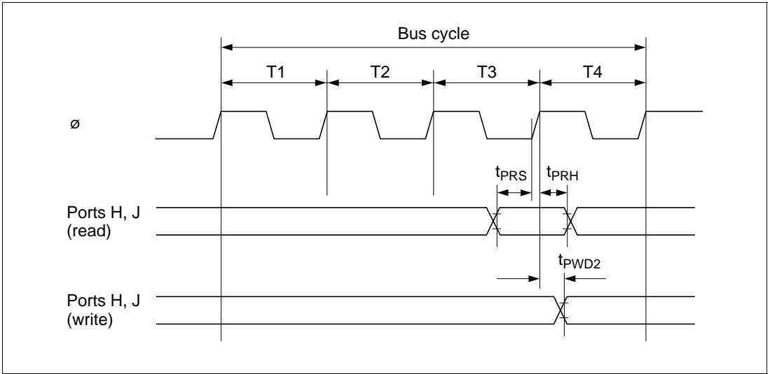
Figure 24-17 I/O Port (Ports H and J) Input/Output Timing
