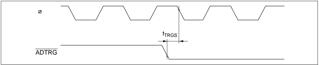
Figure 24-24 A/D Converter External Trigger Input Timing
