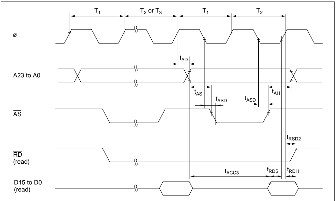
Figure 24-14 Burst ROM Access Timing (Two-State Access)
