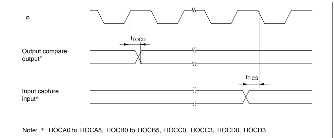
Figure 24-19 TPU Input/Output Timing
