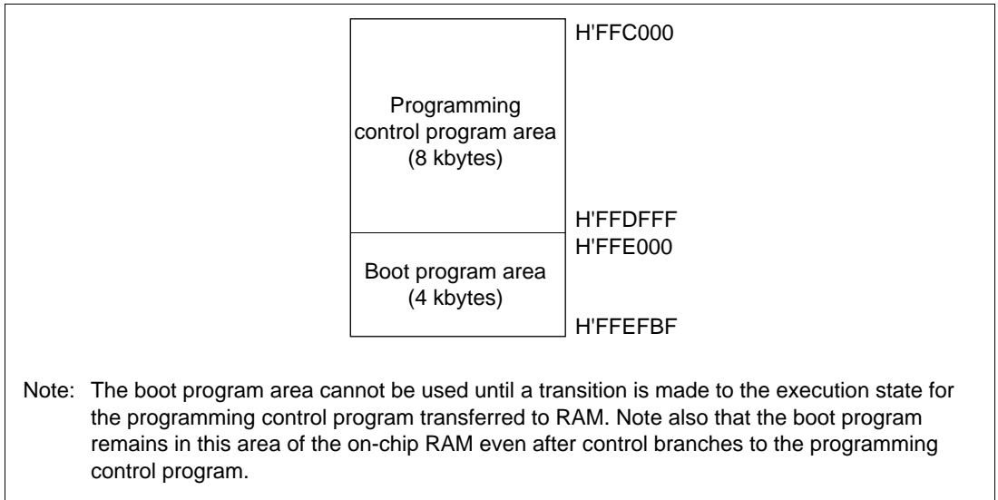
Figure 21B-9 RAM Areas in Boot Mode
