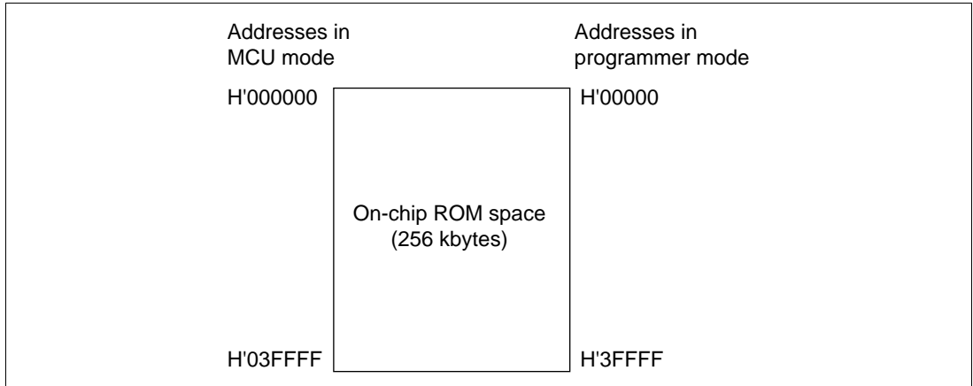
Figure 21B-17 On-Chip ROM Memory Map
