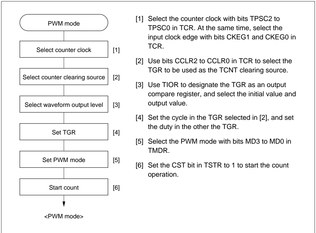
Figure 10-24 Example of PWM Mode Setting Procedure
