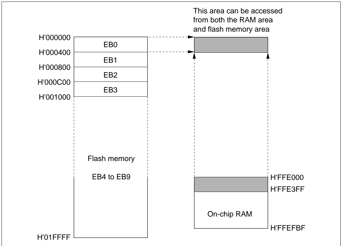
Figure 21A-16 Example of RAM Overlap Operation
