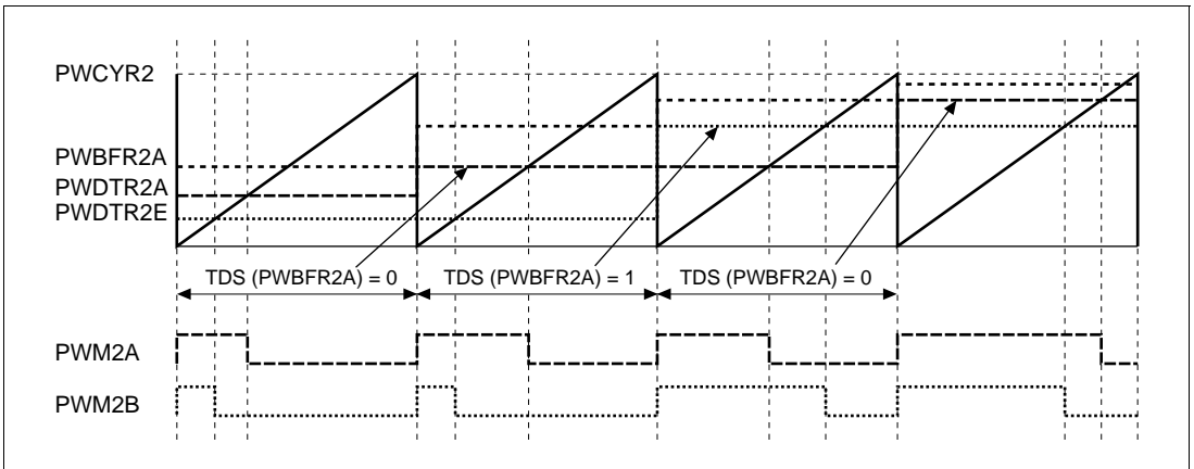
Figure 19-11 PWM Channel 2 Operation
