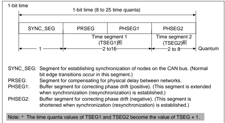
Figure 16-6 Detailed Description of One Bit
