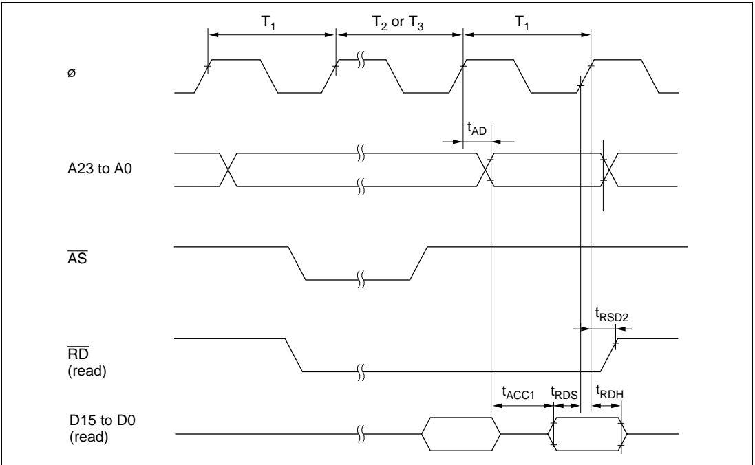
Figure 24-15 Burst ROM Access Timing (One-State Access)
