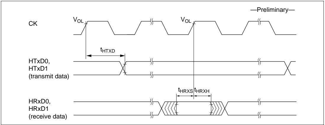
Figure 24-25 HCAN Input/Output Timing
