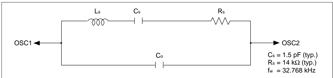
Figure 22A-9 Equivalence Circuit for 32.768kHz Oscillator
