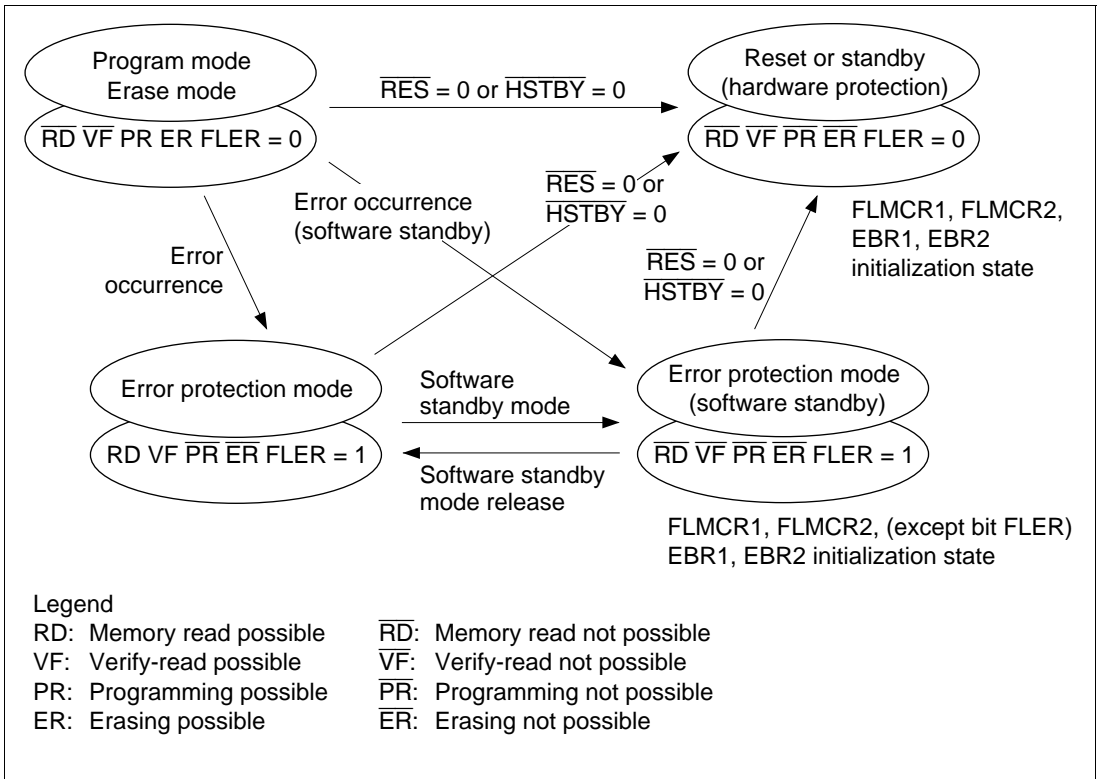
Figure 21B-14 Flash Memory State Transitions
