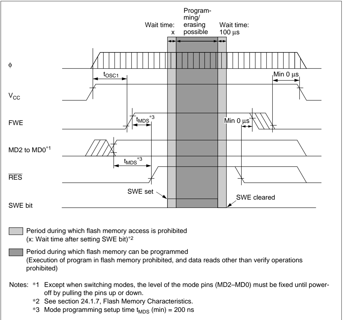
Figure 21A-26 Power-On/Off Timing (Boot Mode)
