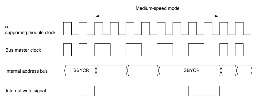
Figure 23B-2 Medium-Speed Mode Transition and Clearance Timing
