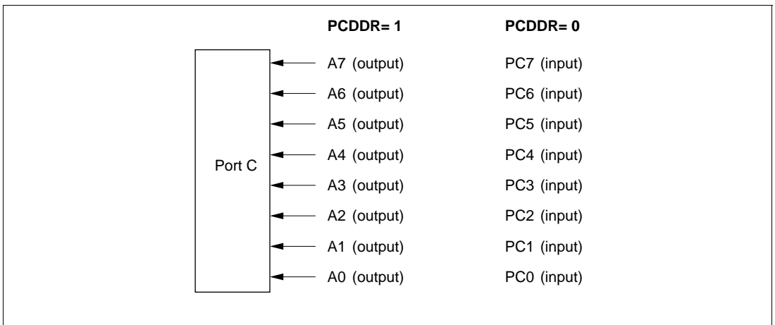
Figure 9-13 Port C Pin Functions (Mode 6)
