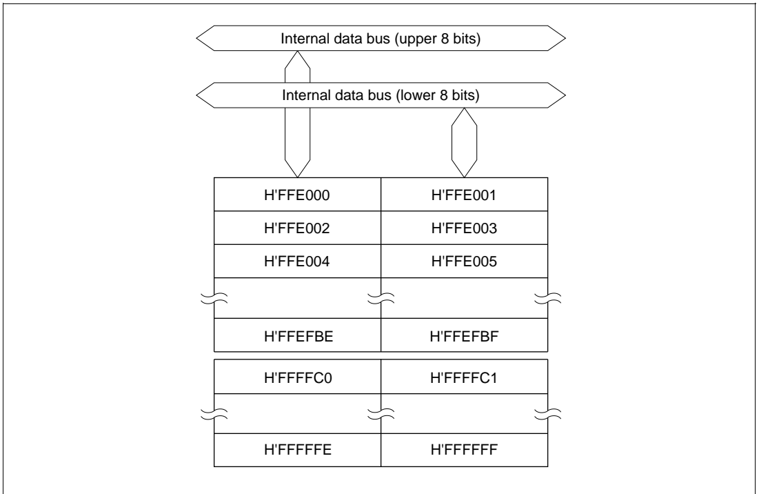
Figure 20-1 (a) Block Diagram of RAM (H8S/2636)
