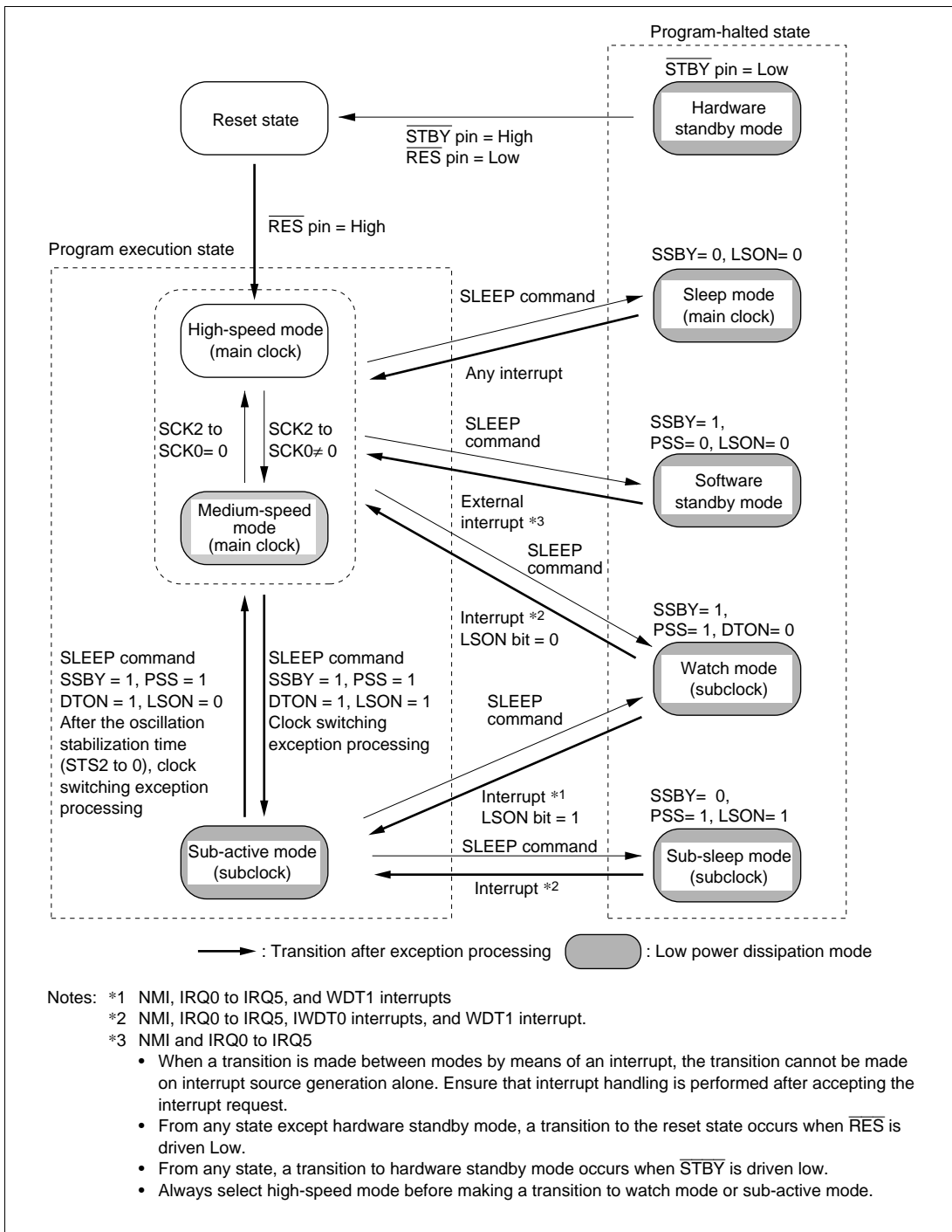
Figure 23B-1 Mode Transition Diagram
