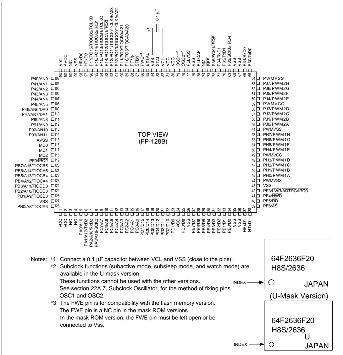
Figure 1-2 Pin Arrangement of HD64F2636F (FP-128B: Top View)
