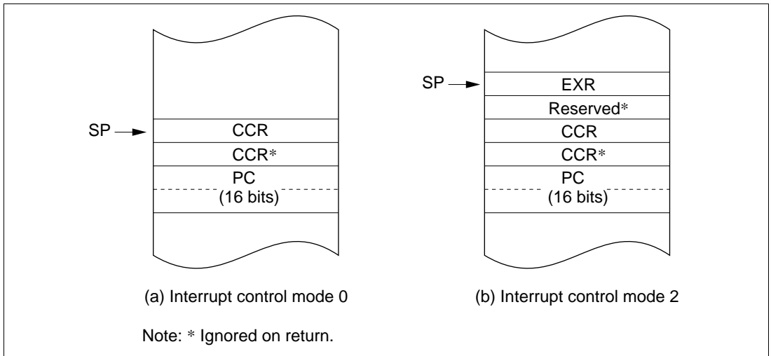
Figure 4-5 (1) Stack Status after Exception Handling (Normal Modes: Not Available in the H8S/2636, H8S/2638, and H8S/2639)
