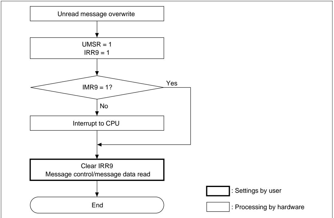
Figure 16-10 Unread Message Overwrite Flowchart
