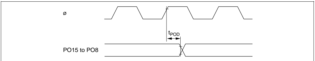
Figure 24-18 PPG Output Timing
