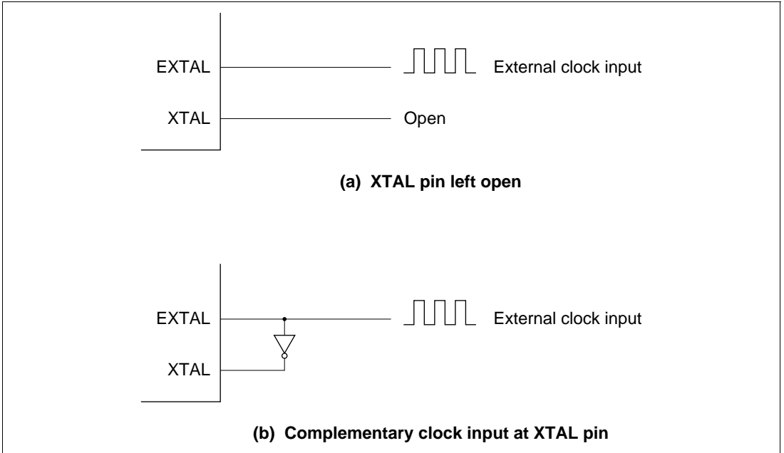
Figure 22B-6 External Clock Input (Examples)
