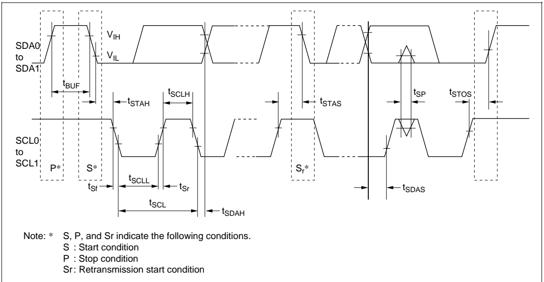
Figure 24-26 I 2 C Bus Interface Input/Output Timing (Option)*
