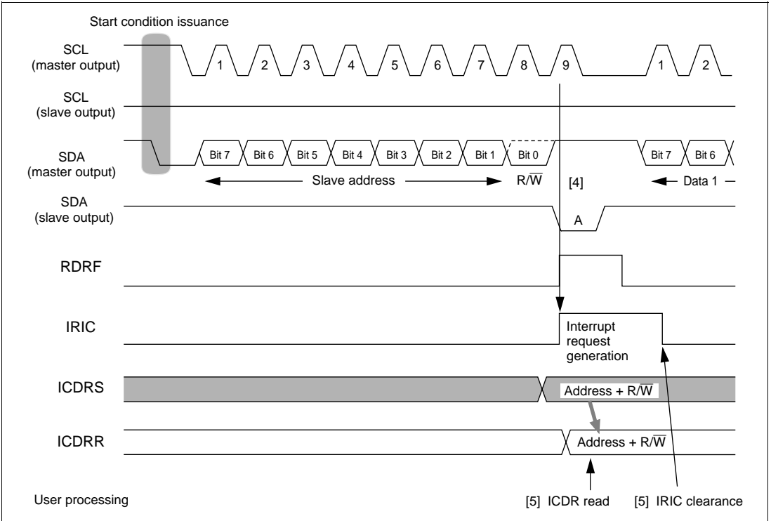
Figure 15-14 Example of Slave Receive Mode Operation Timing (1) (MLS = ACKB = 0)
