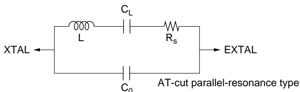
Figure 22B-3 Crystal Resonator Equivalent Circuit
