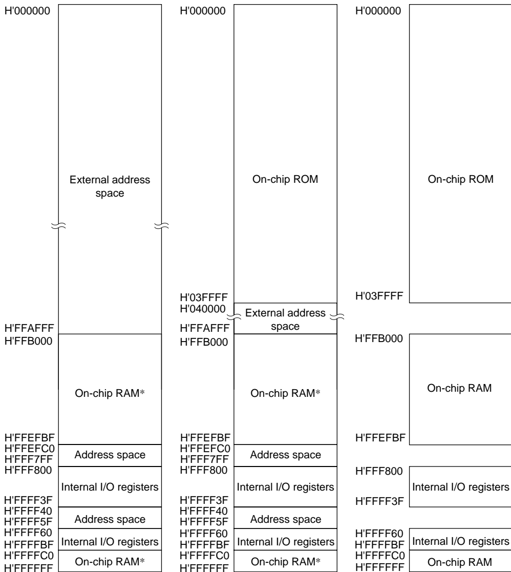
Figure 3-2 Memory Map in Each Operating Mode in the H8S/2638 and H8S/2639
