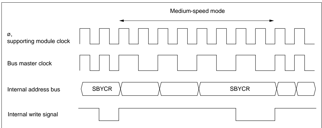
Figure 23A-2 Medium-Speed Mode Transition and Clearance Timing
