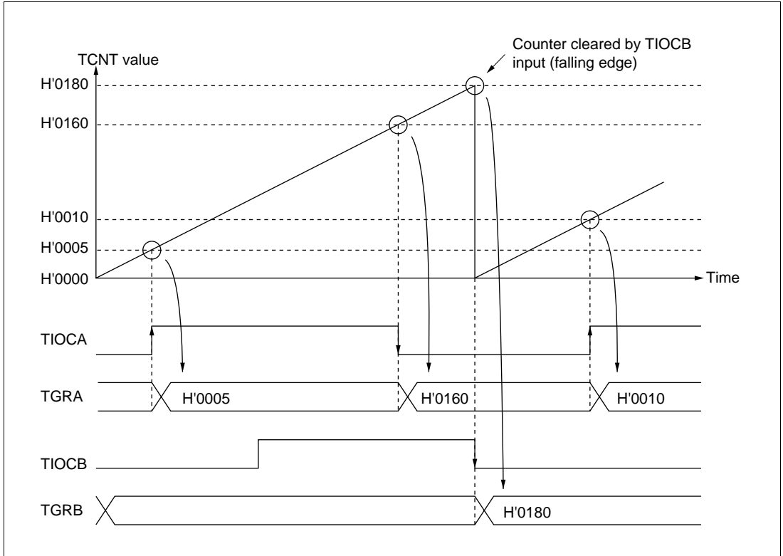
Figure 10-13 Example of Input Capture Operation
