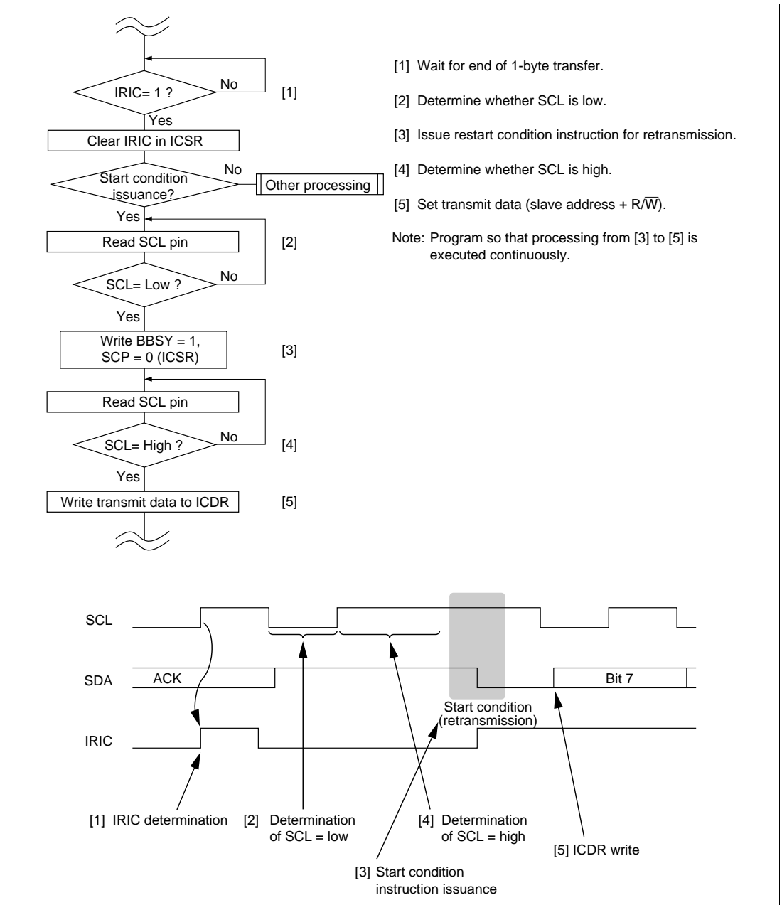
Figure 15-22 Flowchart and Timing of Start Condition Instruction Issuance for Retransmission
