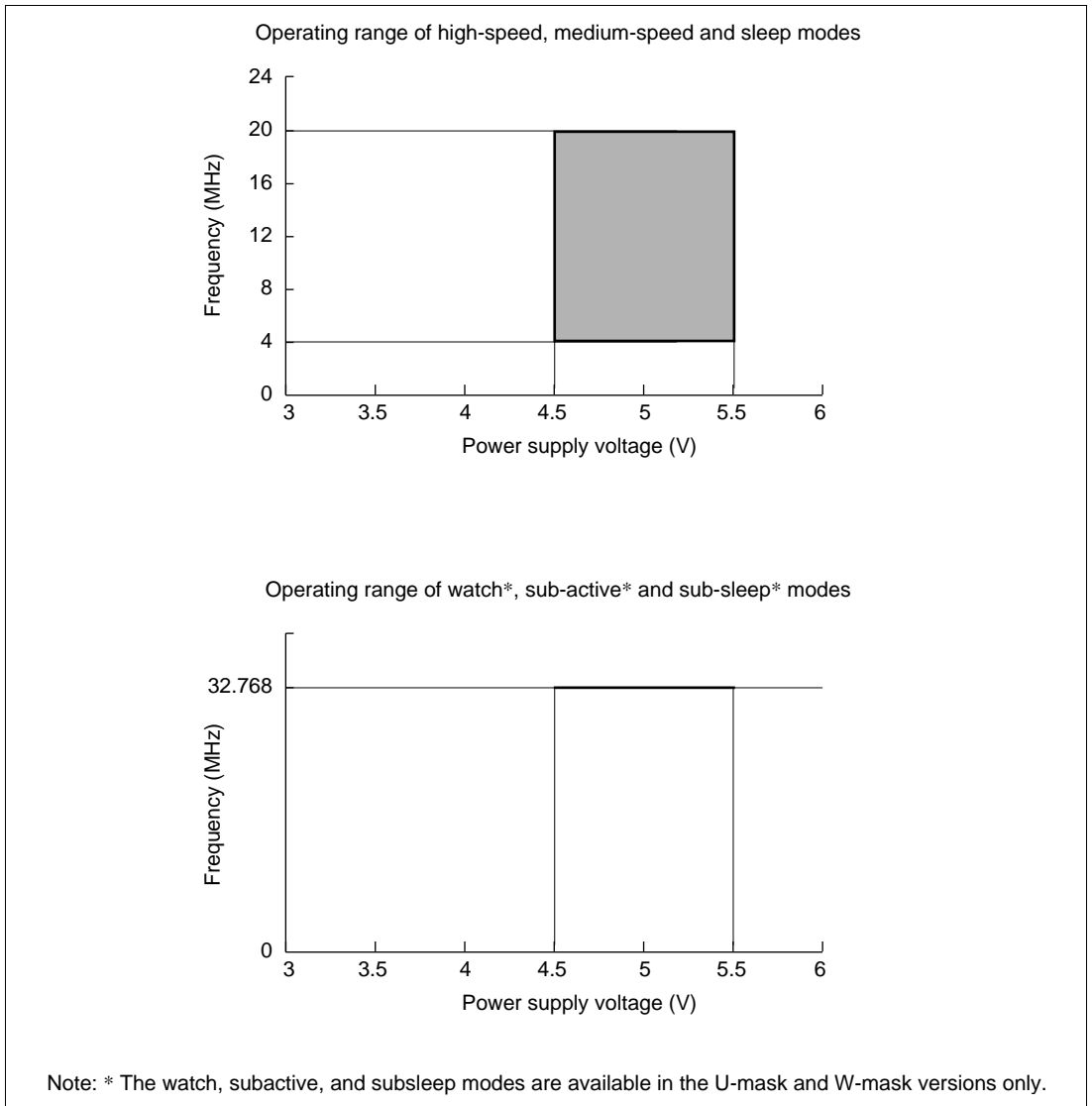
Figure 24-3 Power Supply Voltage and Operating Ranges+
