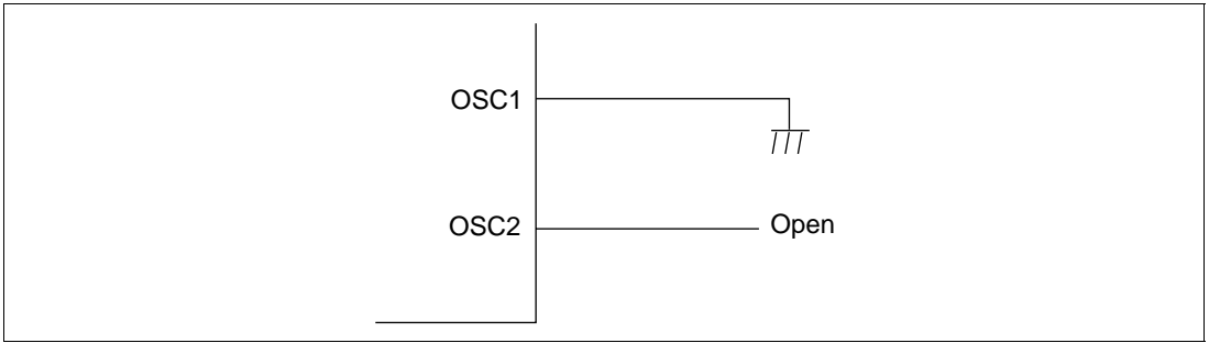
Figure 22A-10 Pin Handling When Subclock Not Required
