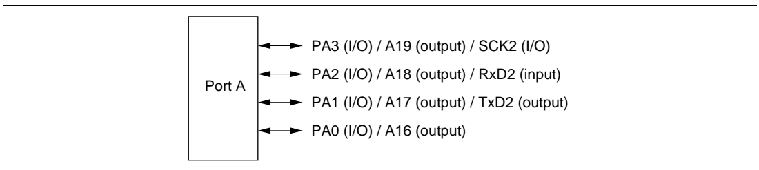
Figure 9-6 Port A Pin Functions (Modes 4 to 6)
