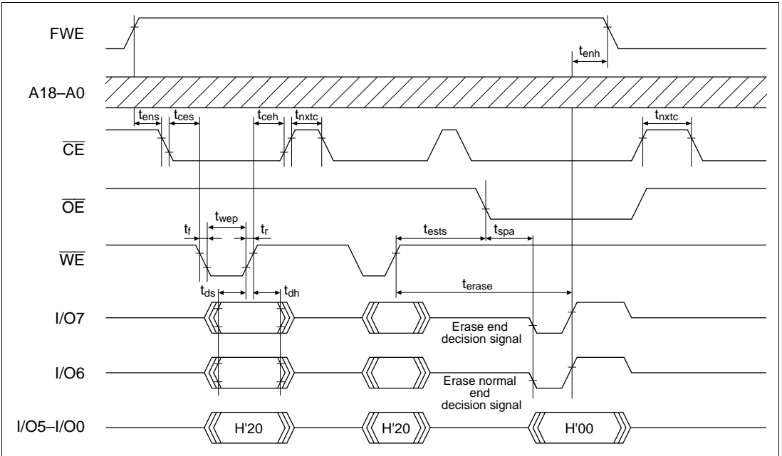
Figure 21B-23 Auto-Erase Mode Timing Waveforms
