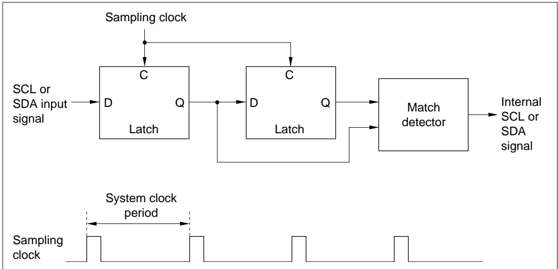
Figure 15-18 Block Diagram of Noise Canceler
