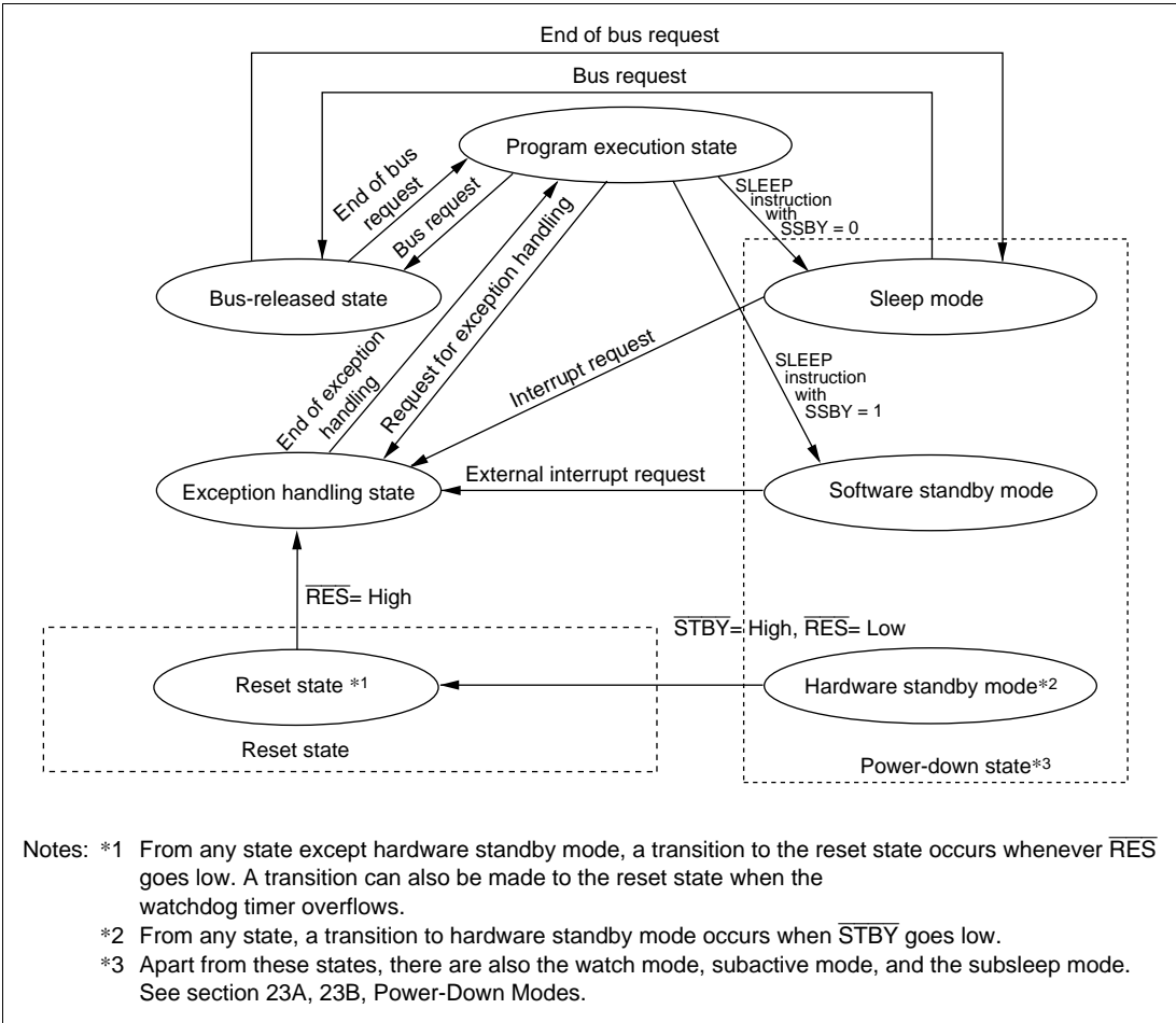
Figure 2-15 State Transitions
