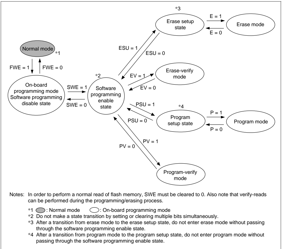
Figure 21A-11 FLMCR1 Bit Settings and State Transitions
