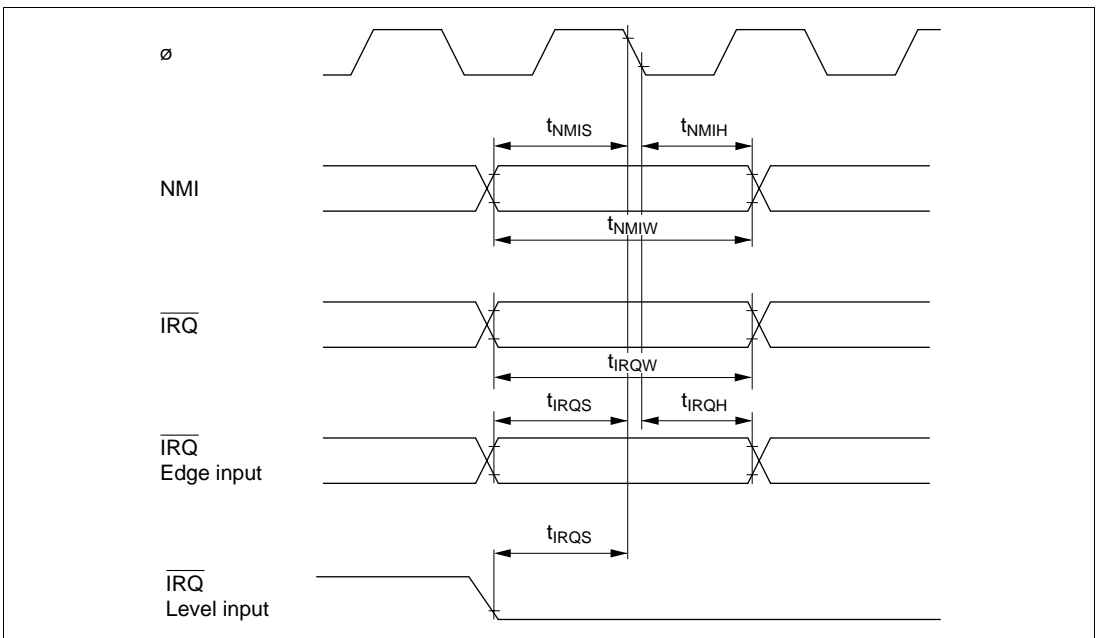
Figure 24-10 Interrupt Input Timing
