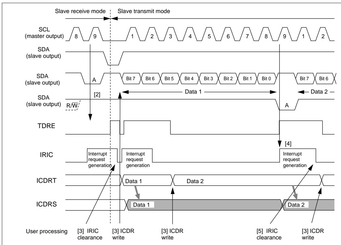
Figure 15-16 Example of Slave Transmit Mode Operation Timing (MLS = 0)
