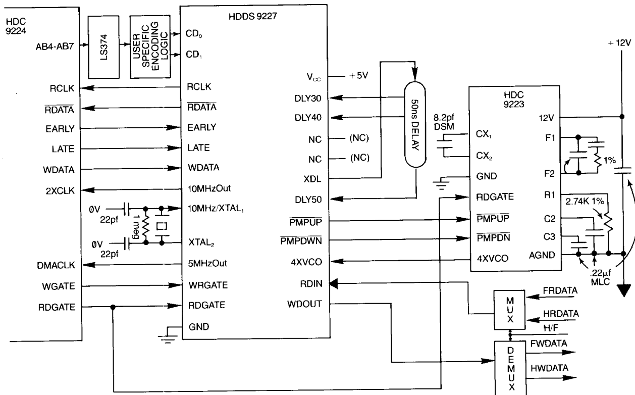
TYPICAL CIRCUIT CONFIGURATION SCHEMATIC 2
