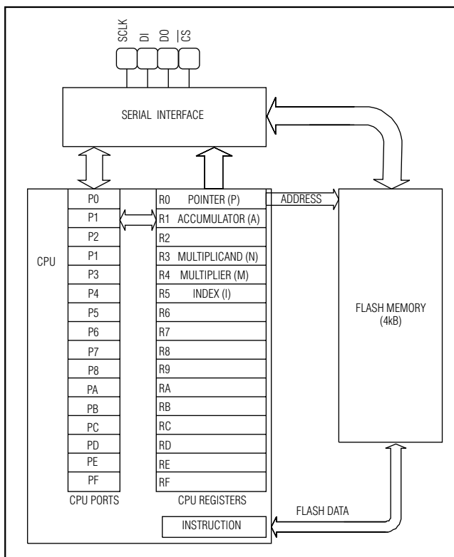
Figure 3. CPU Architecture
