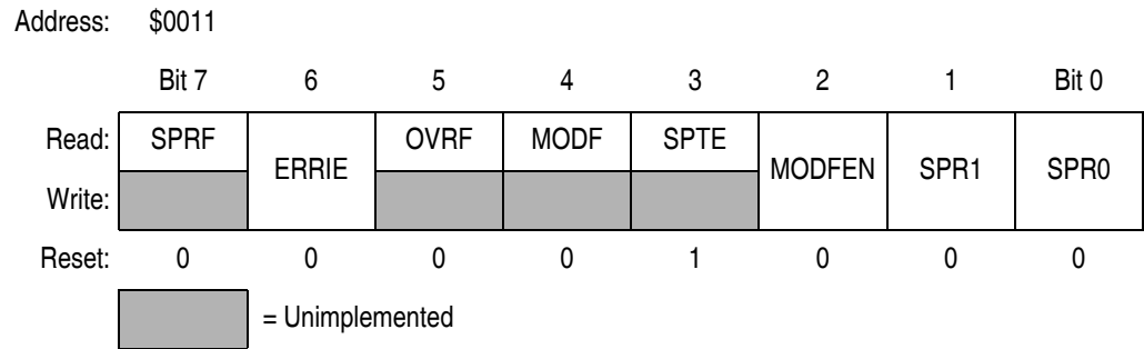
Figure 18-13. SPI Status and Control Register (SPSCR)
