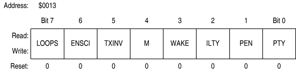
Figure 17-6. SCI Control Register 1 (SCC1)
