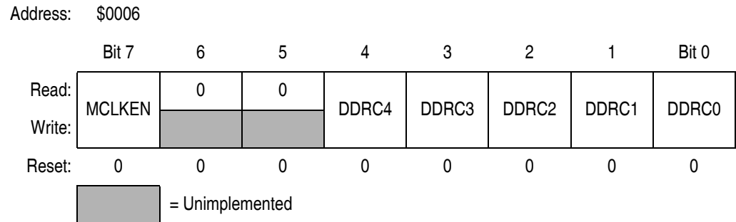
Figure 15-8. Data Direction Register C (DDRC)
