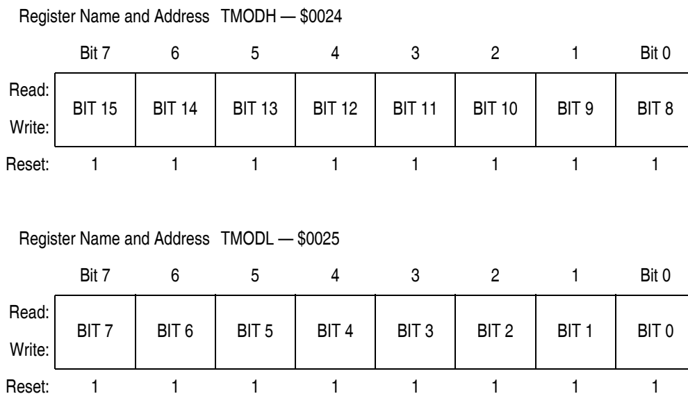
Figure 16-5. TIM Counter Modulo Registers (TMODH and TMODL)
