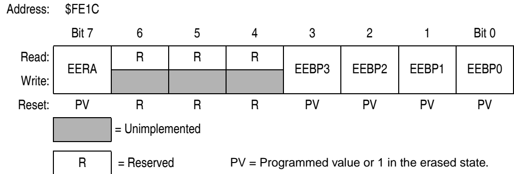
Figure 6-3. EEPROM Nonvolatile Register (EENVR)
