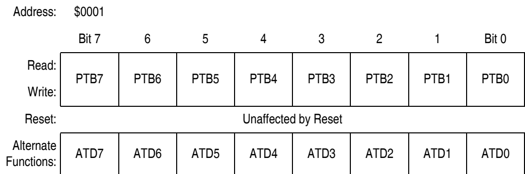
Figure 15-4. Port B Data Register (PTB)
