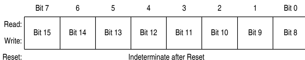
Figure 16-8. TIM Channel Registers (TCH0H/L–TCH3H/L) (Sheet 1 of 3)
