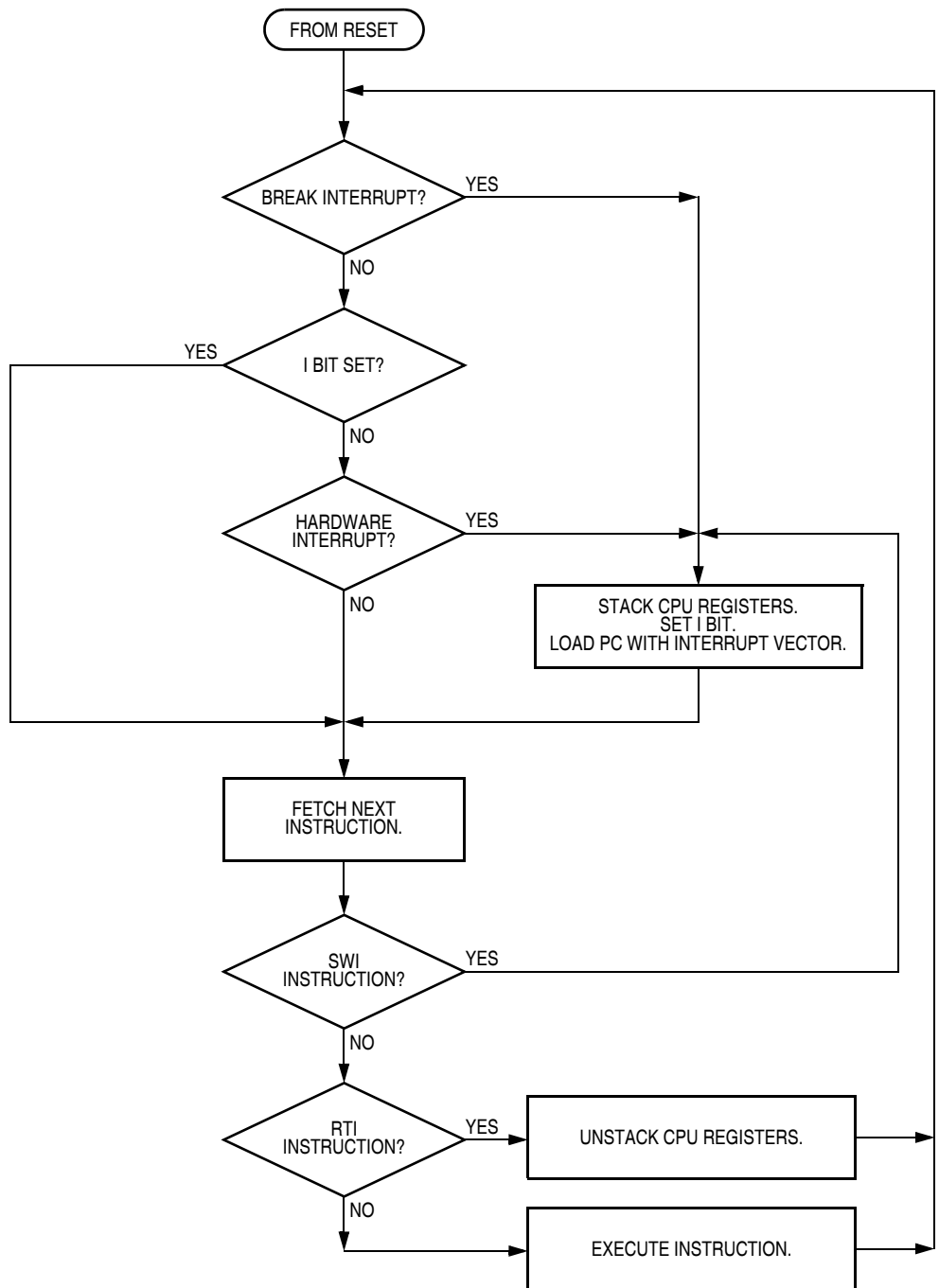
Figure 9-8. Interrupt Processing
