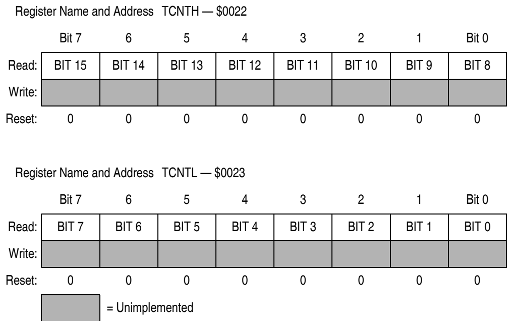
Figure 16-4. TIM Counter Registers (TCNTH and TCNTL)
