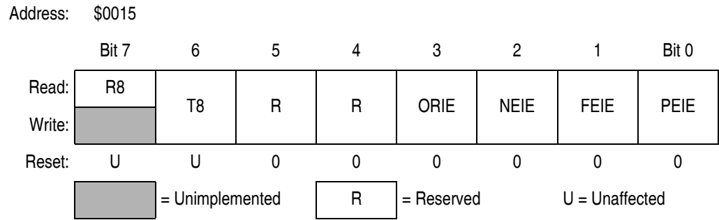
Figure 17-8. SCI Control Register 3 (SCC3)
