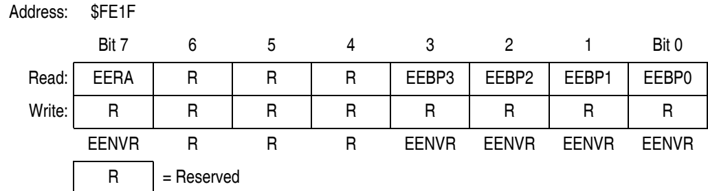
Figure 6-2. EEPROM Array Control Register (EEACR)
