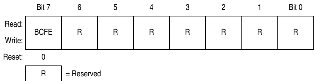
Figure 9-18. SIM Break Flag Control Register (SBFCR)
