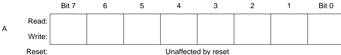
Figure 1. Accumulator (A)
