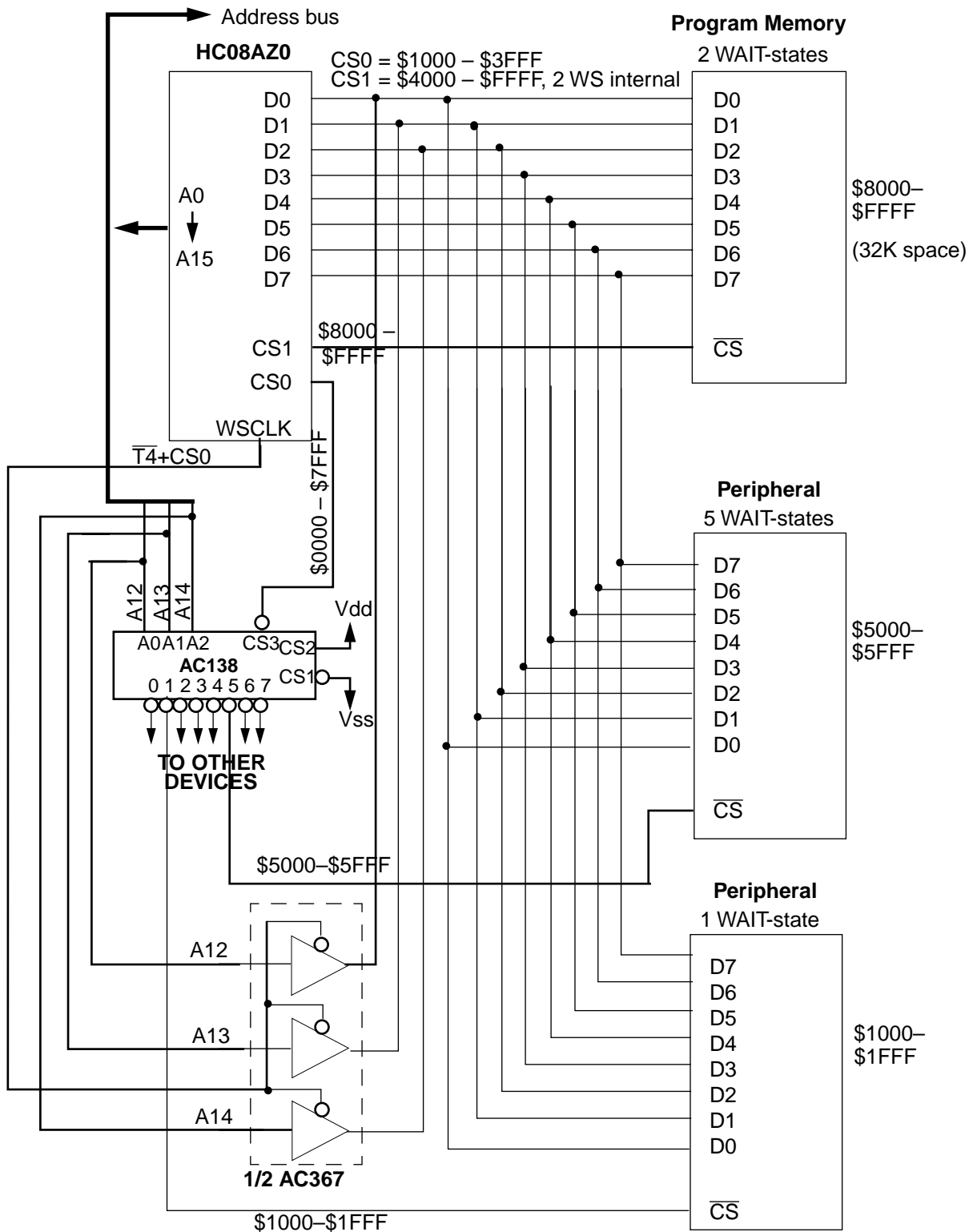
Figure 10 WAIT state selection for multiple I/O peripherals
