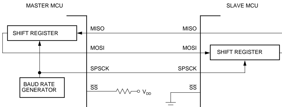
Figure 3. Full-duplex master-slave connections
