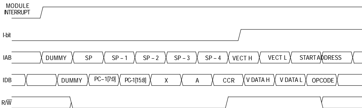
Figure 7. Interrupt entry
