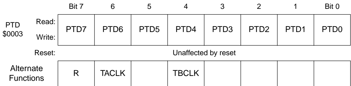
Figure 10. Port D data register (PTD)
