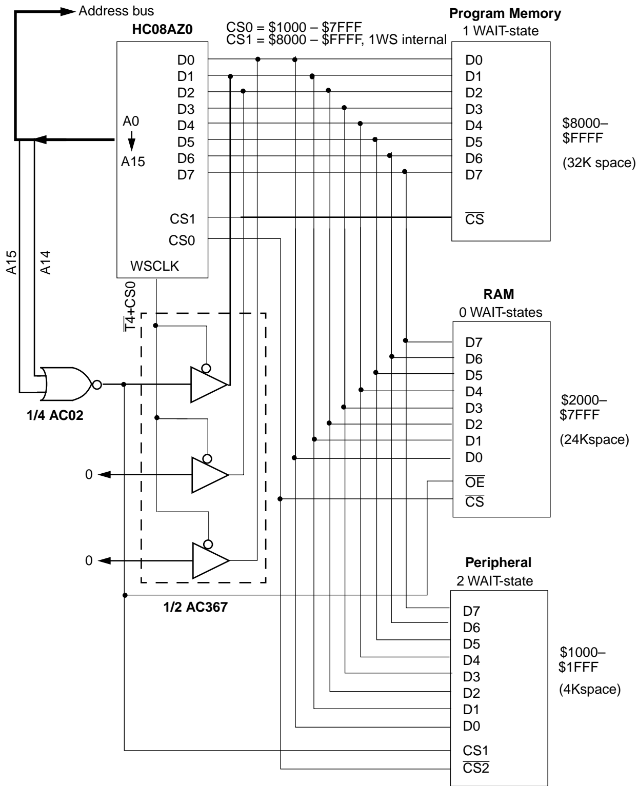
Figure 9 Simple address space decode with different WAIT states
