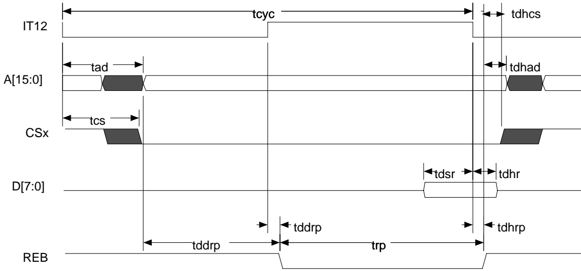
Figure 3 High performance read timings
