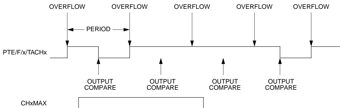
Figure 7. CHxMAX Latency
