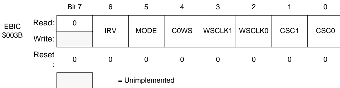
Figure 11 EBI control register (EBIC)
