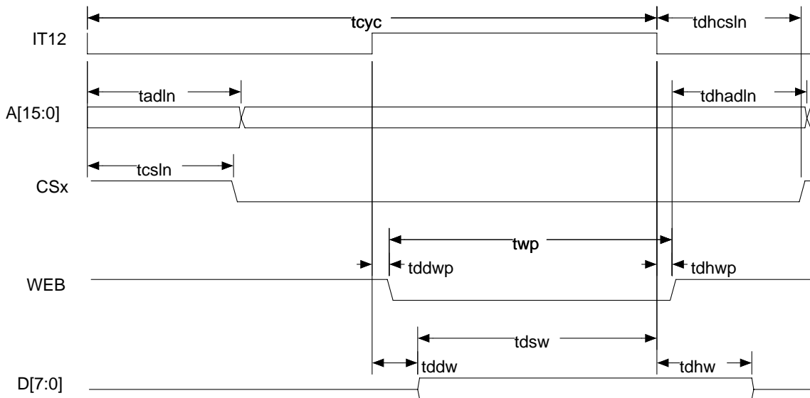
Figure 6 Low-noise mode write timings
