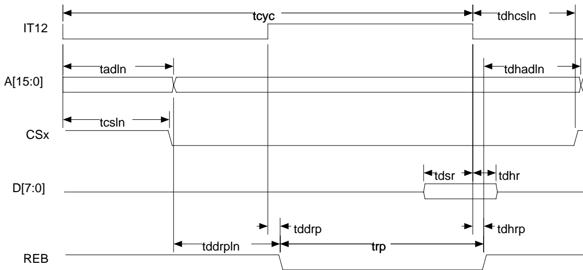
Figure 5 Low noise mode read timings
