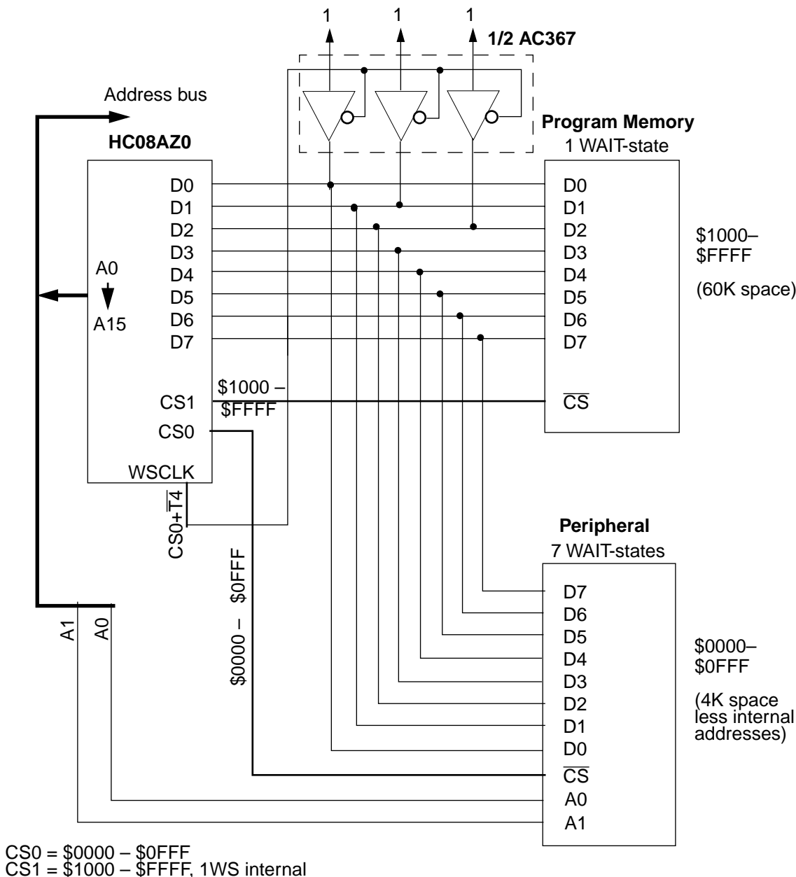
Figure 8 Defining WAIT states for Ext addresses below $1000
