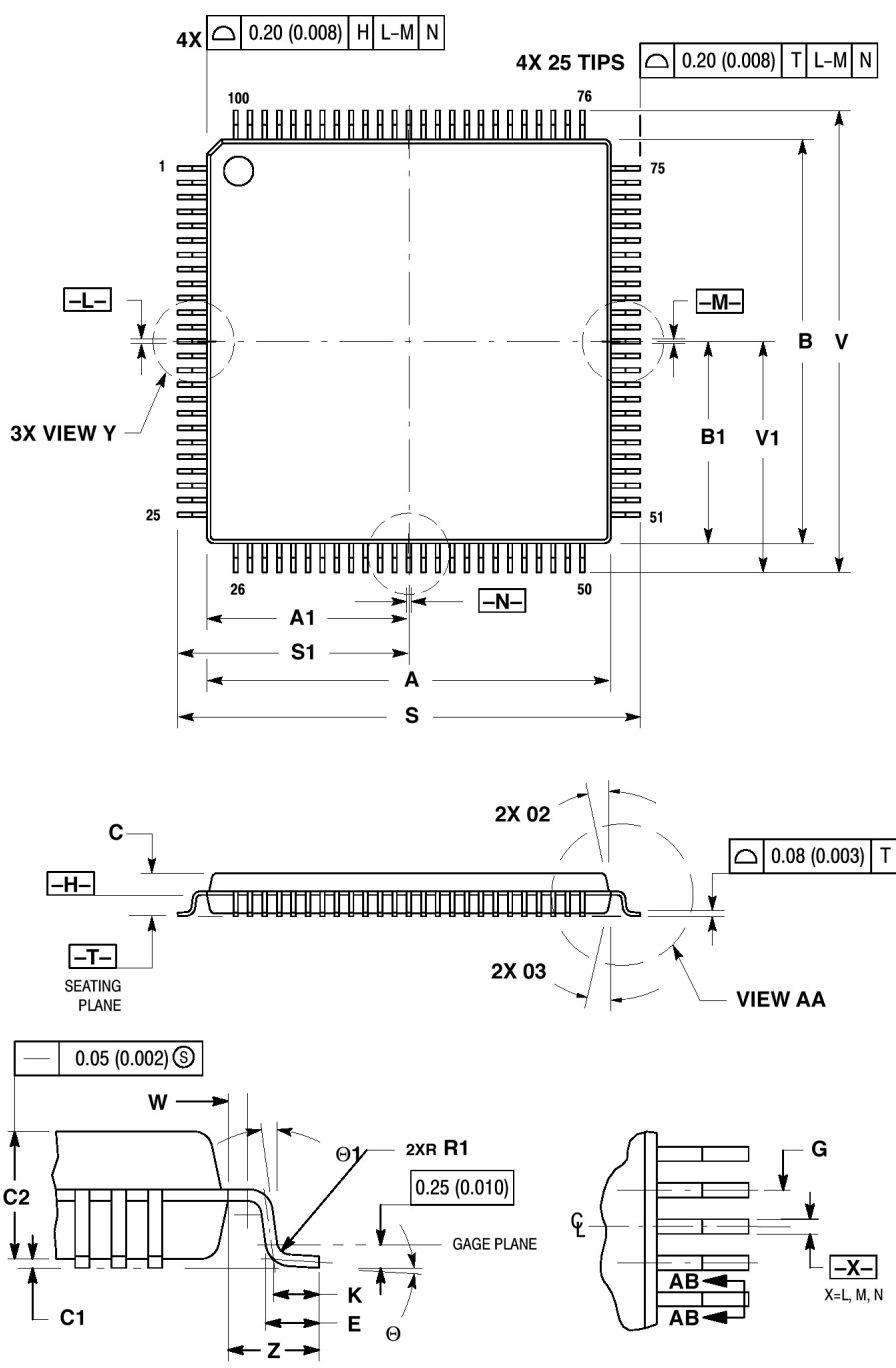
Figure 7. 100-pin QFP
