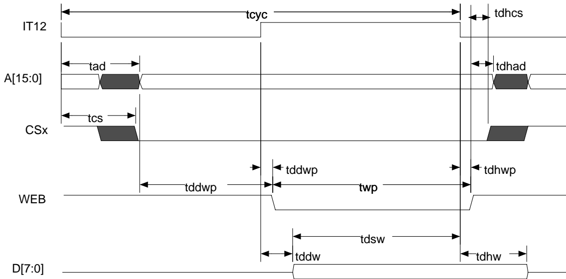
Figure 4 High performance write timings
