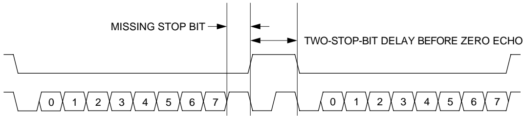
Figure 5. Break transaction
