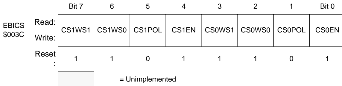
Figure 12 EBI control register (EBICS)
