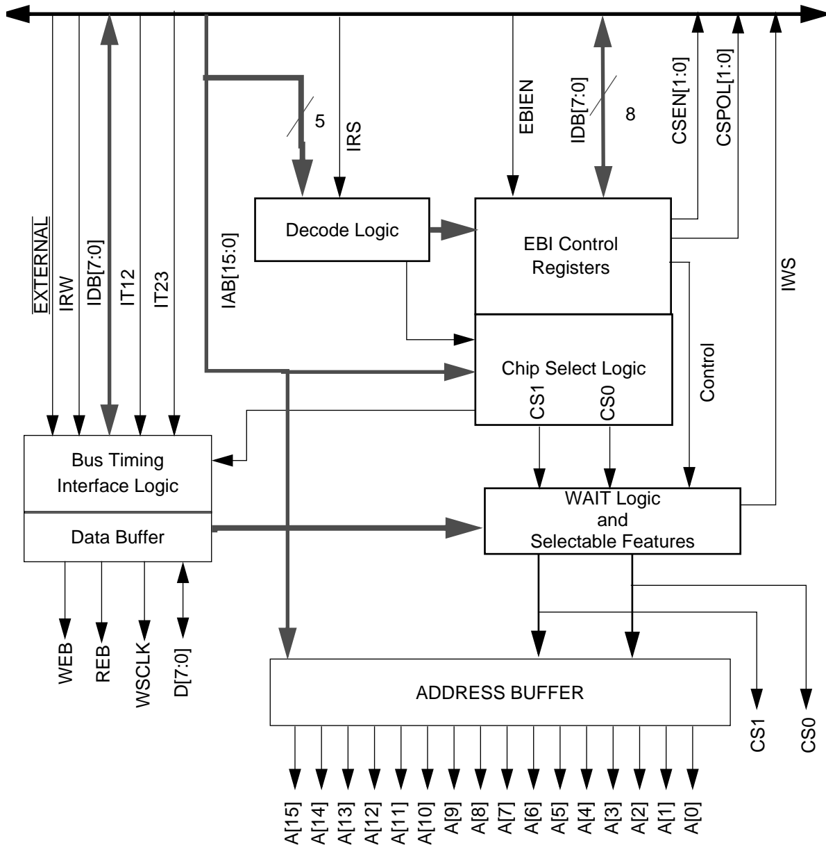
Figure 6 EBI Block Diagram
