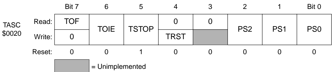
Figure 3. TIMA status and control register (TASC)
