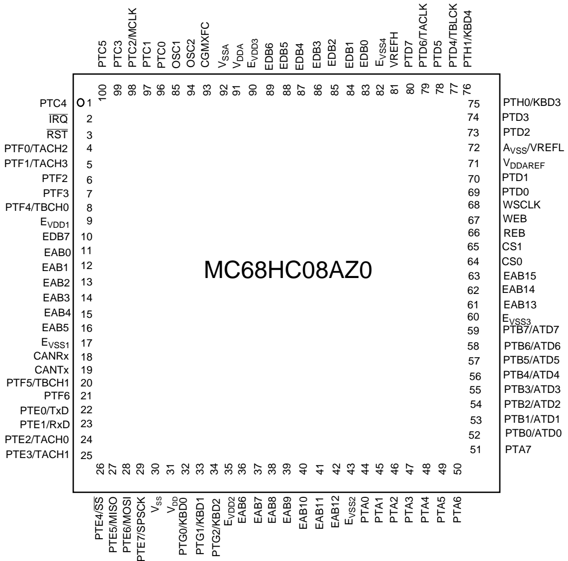
Figure 2. 100 QFP pin assignments
