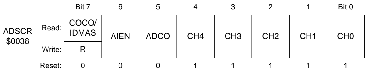
Figure 2. ADC status and control register
