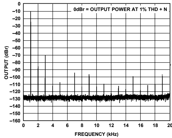
Figure 14. FFT, 1 W, 15 V, 8 Ω
