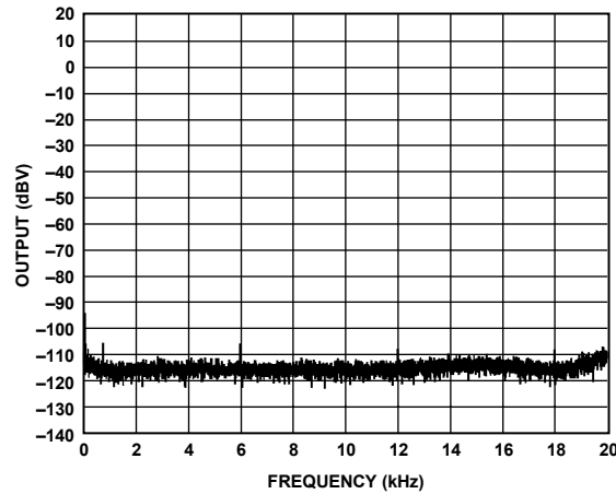
Figure 16. FFT Dither, 15 V, 8 Ω
