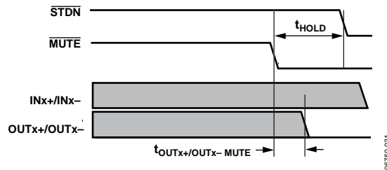
Figure 3. Timing Diagram Mute
