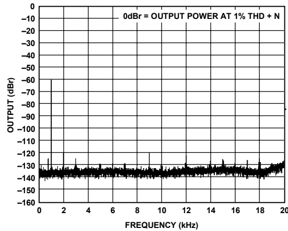
Figure 15. FFT, 60 dBFS, 15 V, 8 Ω
