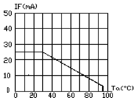
FIG.5 MAXIMUM FORWARD CURRENT VS. AMBIENT TEMPERATURE (Tjmax=105°C)
