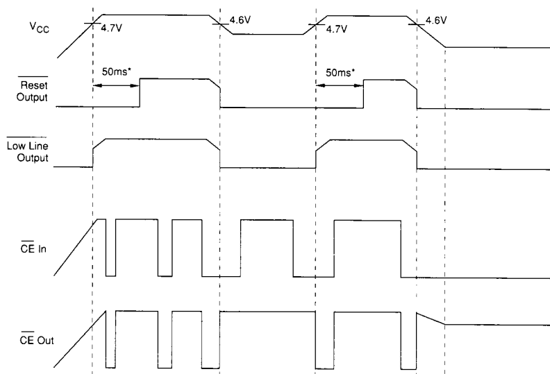
Figure 6. Reset Timing
