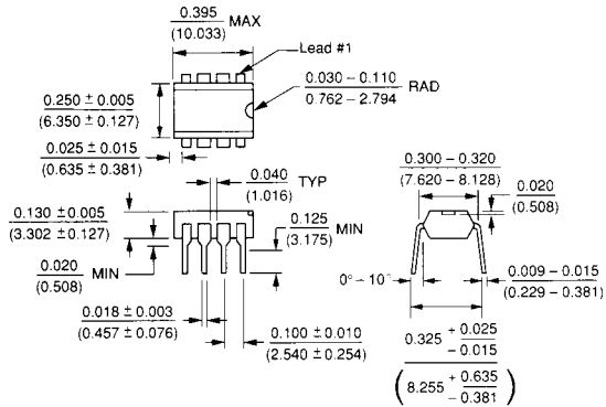
8 LEAD PLASTIC DIP (P)
