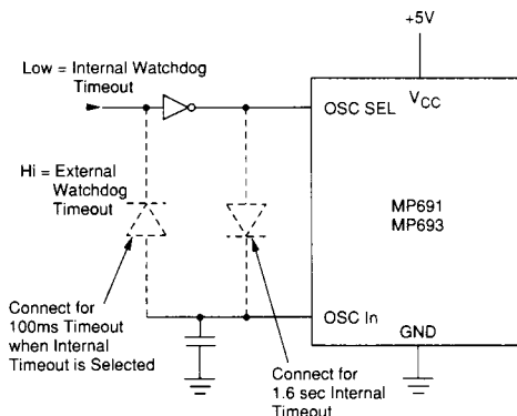
Figure 14. Selecting Internal or External Watchdog Timeout
