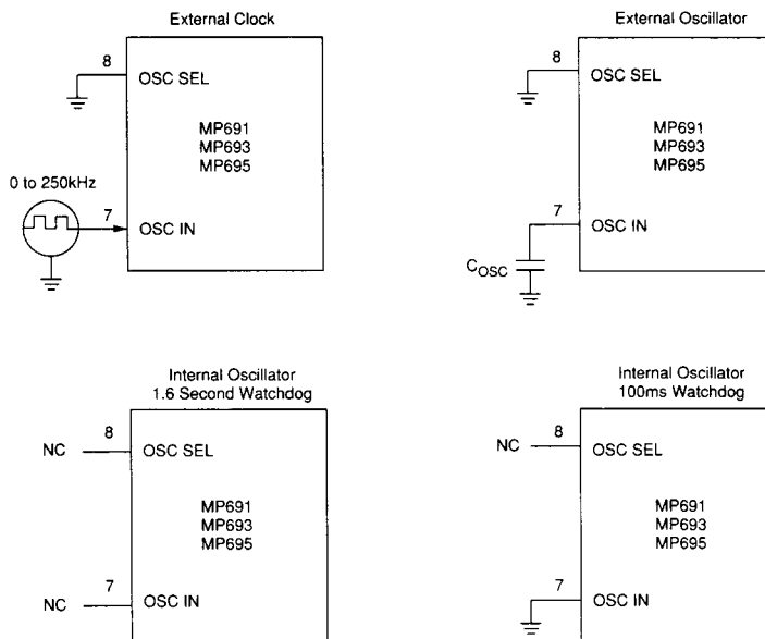
Figure 8. Oscillator Circuits
