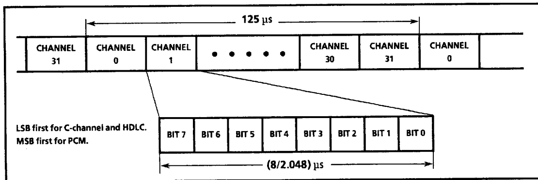
Figure 8 - Format of ST-BUS Stream
