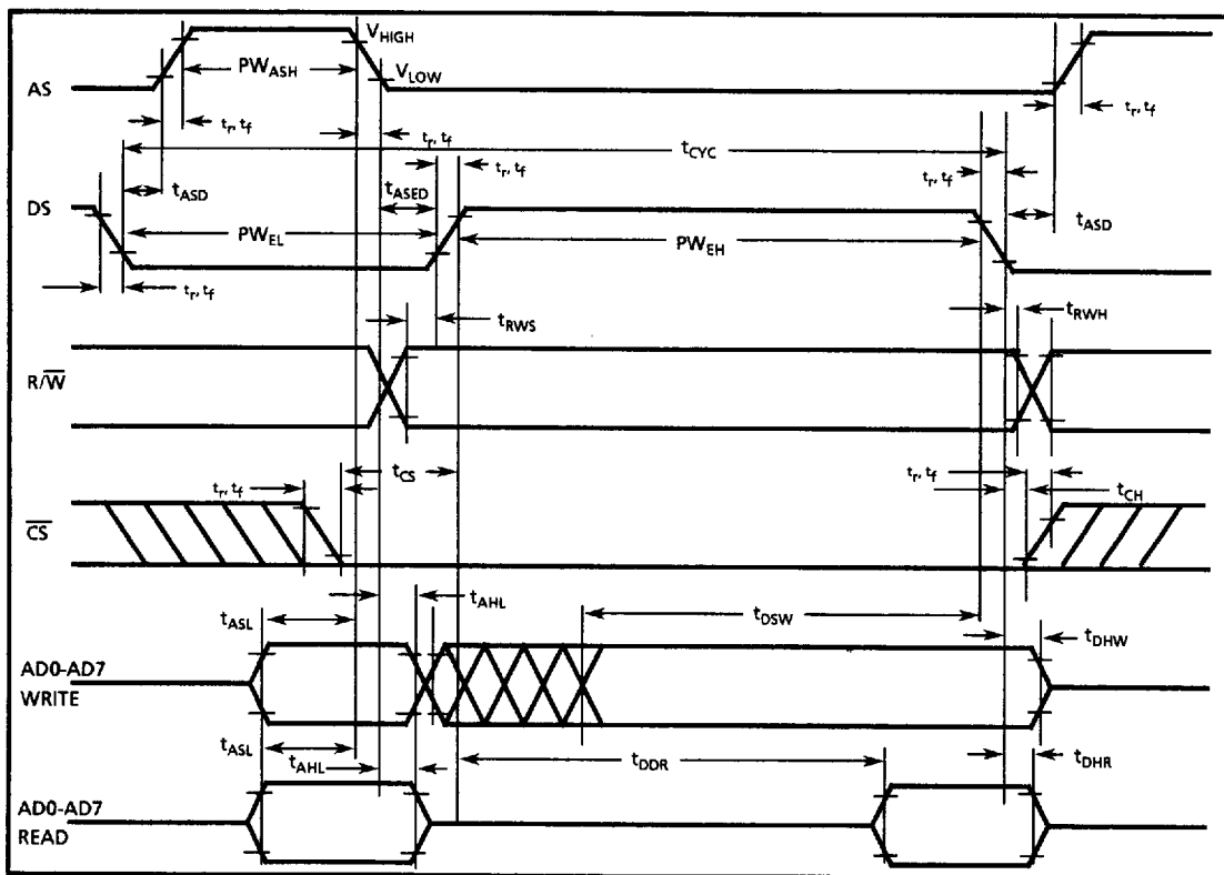
Figure 13 - Motorola BUS Timing
