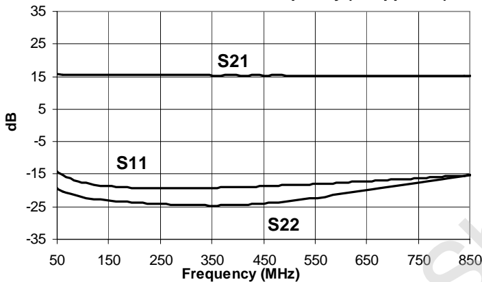
Gain & Return Loss vs. Frequency (w/ App. Ckt.)
