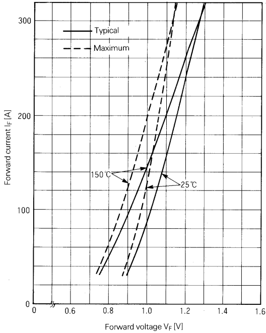
Forward Characteristics
