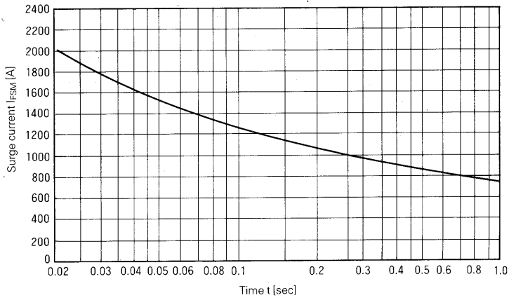
Surge Current
