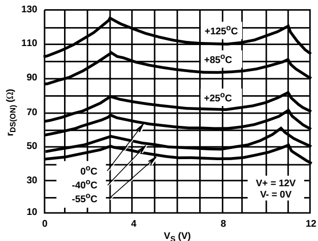
r_{DS(ON)} vs V_S AND TEMPERATURE (SINGLE SUPPLY)
