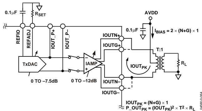
Figure 64. Current-Mode Operation
