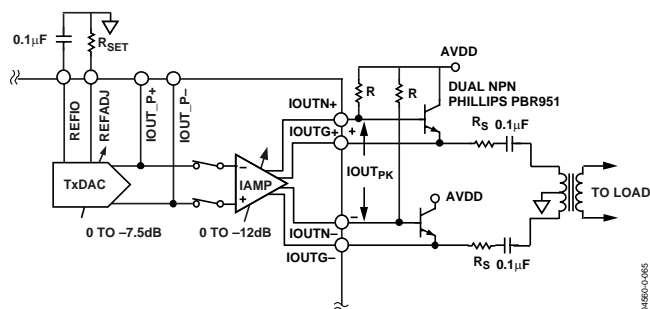
Figure 65. Voltage-Mode Operation
