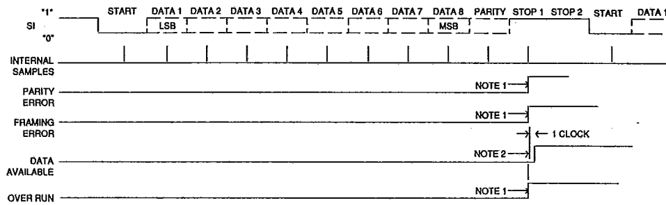
FIG. 6 UART/T - RECEIVER TIMING
