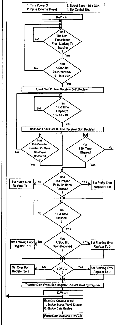
FIG. 23 RECEIVER OPERATION
