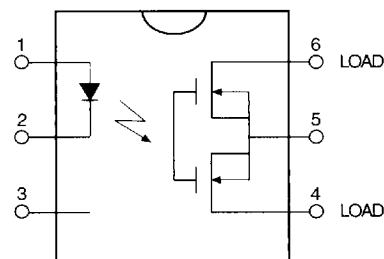
Pin Connections
