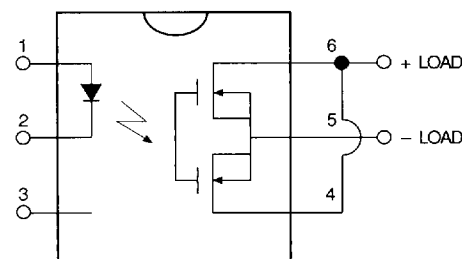
Pin Connections
