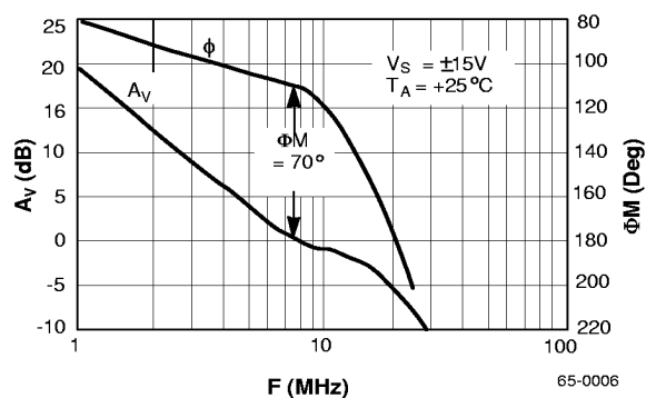
Figure 4. Gain, Phase Shift vs. Frequency
