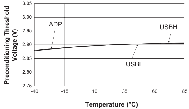
Preconditioning Threshold Voltage vs. Temperature ( V_{IN} = 5.0V )
