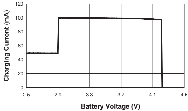
Charging Current vs. Battery Voltage (USBL; USBSET = 71.5kΩ)
