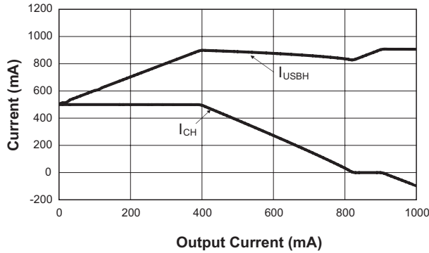
USB and Charging Current vs. Output Current (USBH; V_{BAT} = 3.6V )
