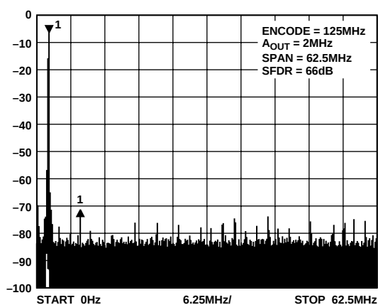
Figure 9. Wideband SFDR 2 MHz A_{OUT} ; 125 MHz Clock
