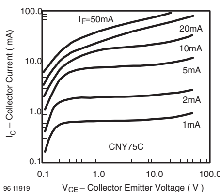
96 11919 Figure 11. Collector Current vs. Collector Emitter Voltage
