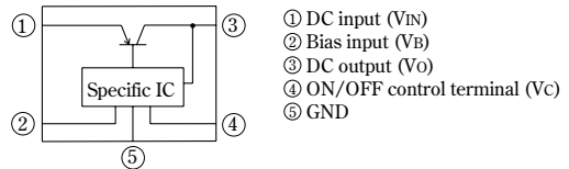
Internal connection diagram
